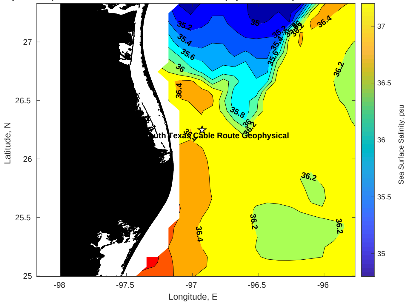
Surface Salinity for Tampnet P2378 South Texas Cable Route Geophysical at 27-Apr-2025 00:00:00
