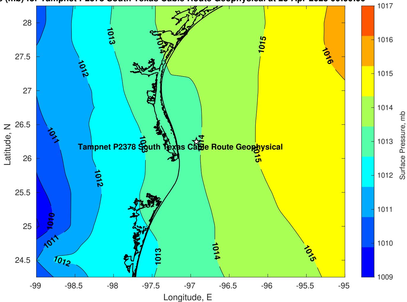
Pressure (mb) for Tampnet P2378 South Texas Cable Route Geophysical at 28-Apr-2025 00:00:00
