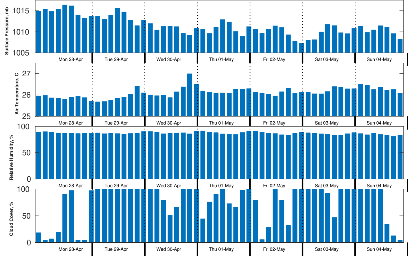
Met Forecast for Tampnet P2378 South Texas Cable Route Geophysical from 28-Apr-2025 00:00:00 to 05-May-2025 00:00:00
