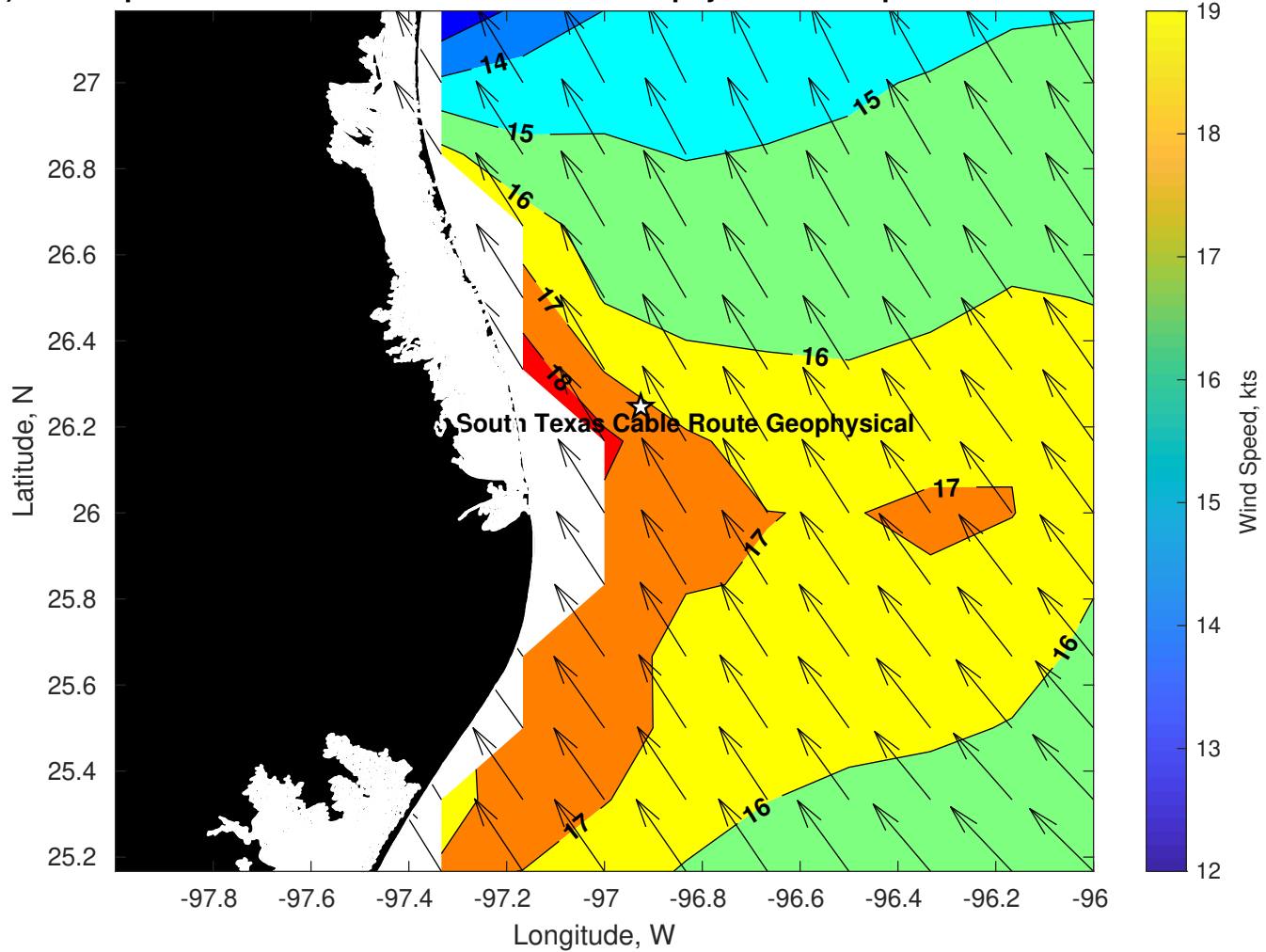
Winds (kts) for Tampnet P2378 South Texas Cable Route Geophysical at 28-Apr-2025 09:00:00
