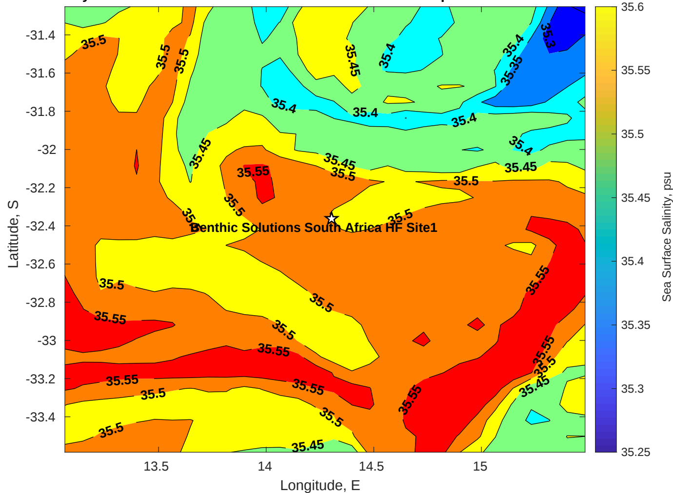
Surface Salinity for Benthic Solutions South Africa HF Site1 at 28-Apr-2025 00:00:00
