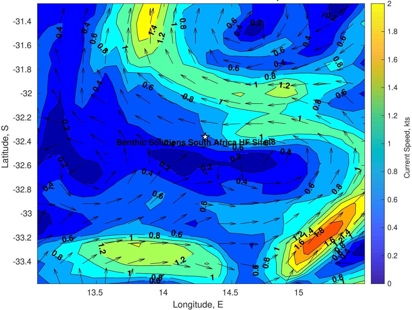
Surface Currents for Benthic Solutions South Africa HF Site1 at 28-Apr-2025 00:00:00
