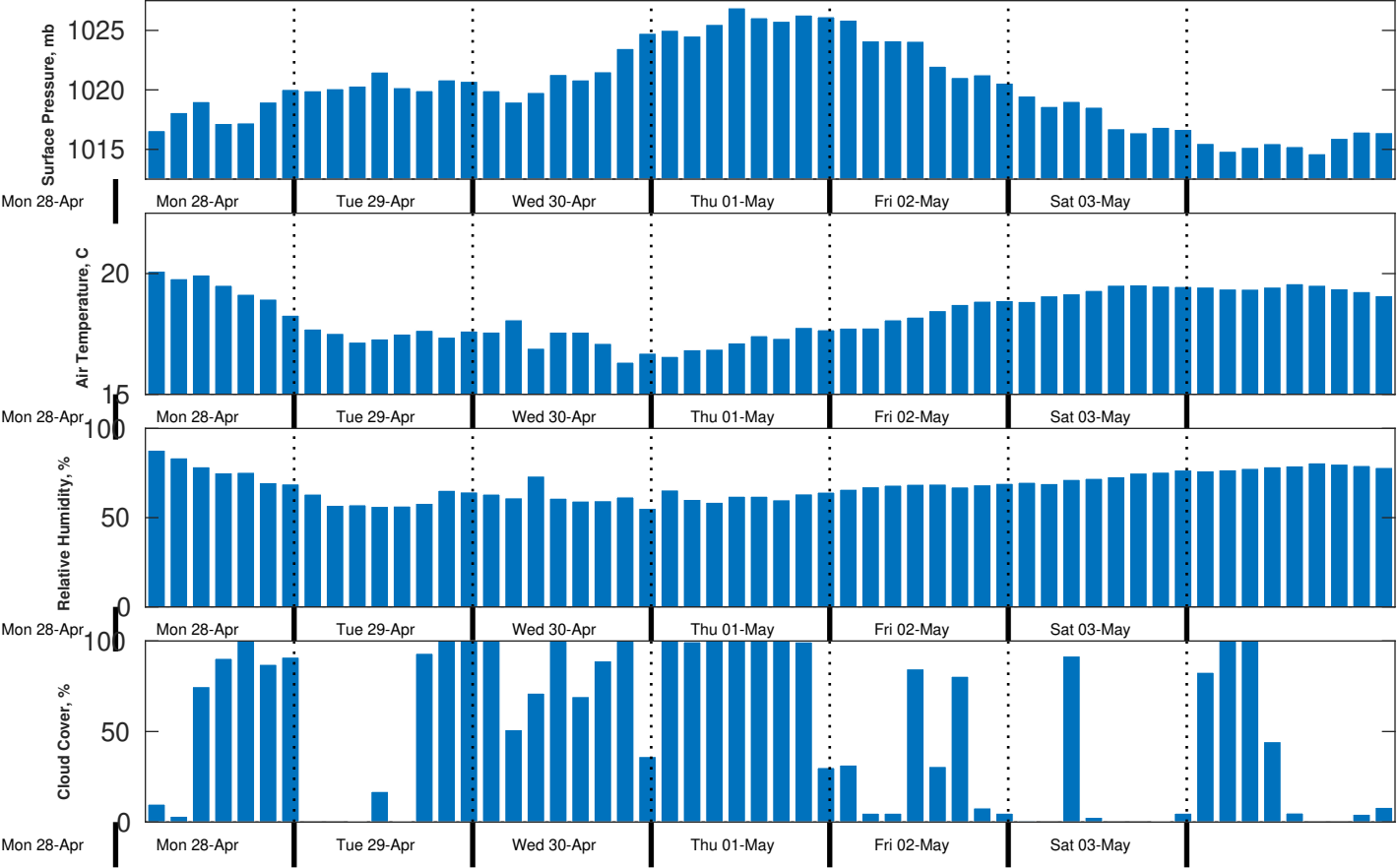
Met Forecast for Benthic Solutions South Africa HF Site1 from 29-Apr-2025 00:00:00 to 06-May-2025 00:00:00
