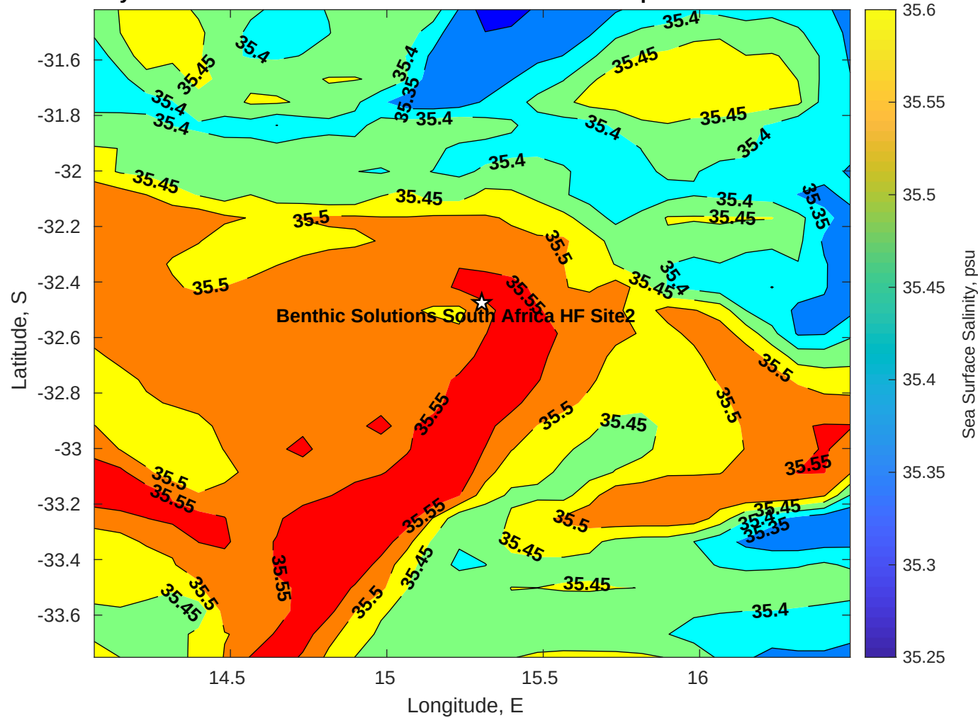
Surface Salinity for Benthic Solutions South Africa HF Site2 at 28-Apr-2025 00:00:00
