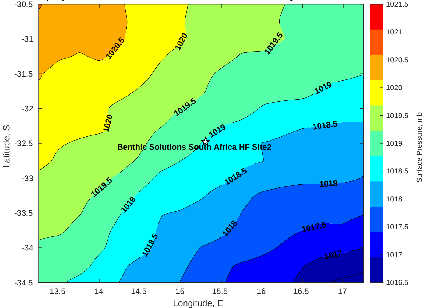
Surface Pressure (mb) for Benthic Solutions South Africa HF Site2 at 01-May-2025 00:00:00
