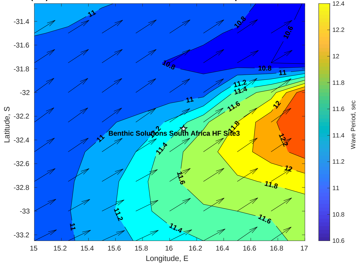
Wave Period (sec) for Benthic Solutions South Africa HF Site3 at 29-Apr-2025 09:00:00
