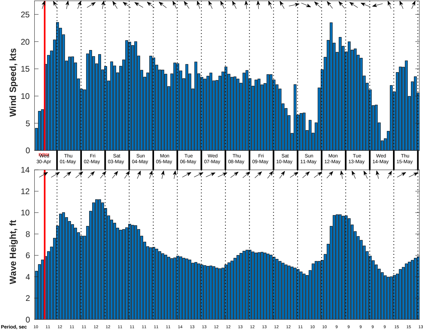
Wind & Wave Forecast for Benthic Solutions South Africa HF Site3 from 29-Apr-2025 02:00:00 to 15-May-2025 02:00:00
