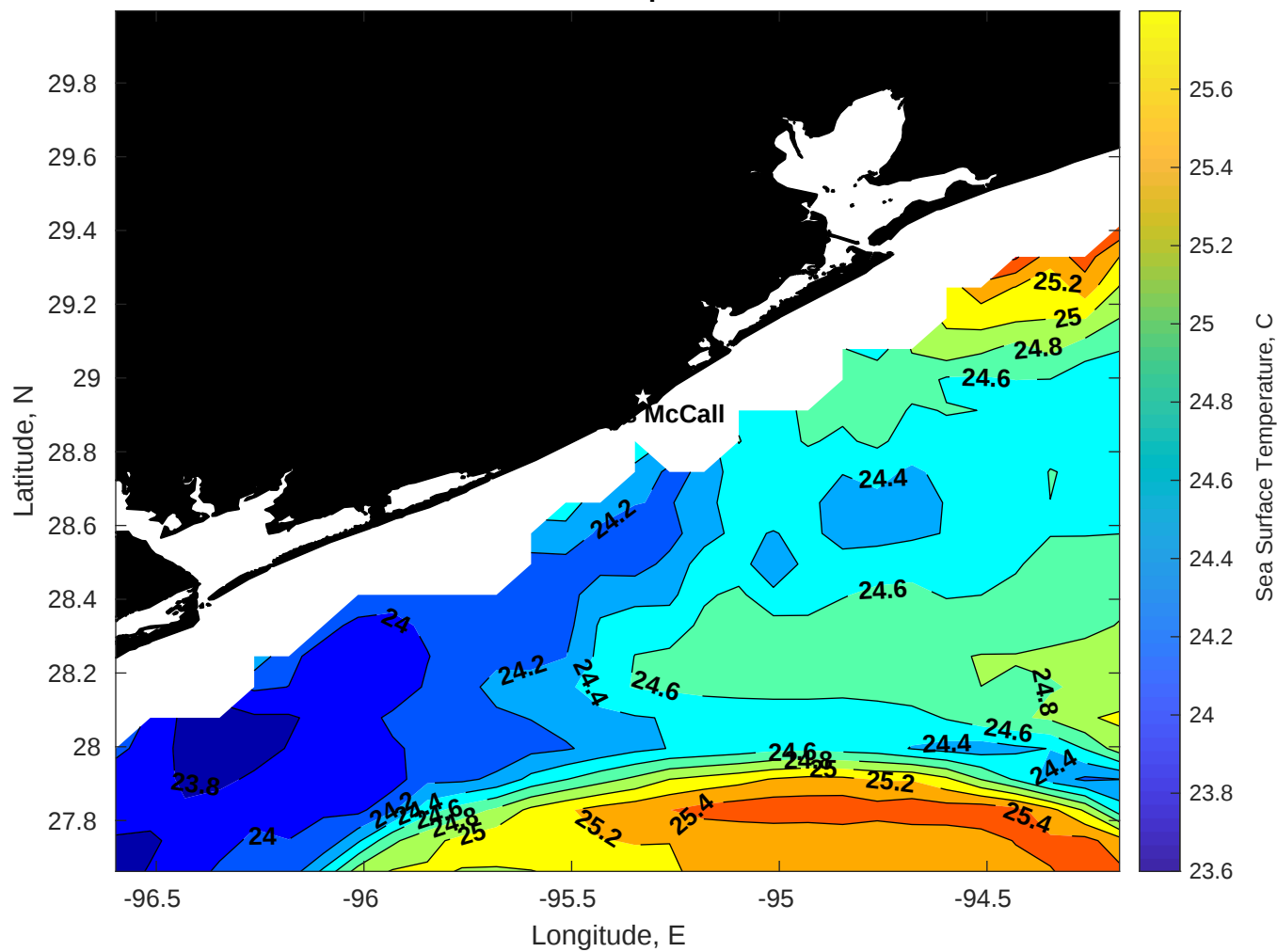
SST for Brooks McCall at 28-Apr-2025 00:00:00
