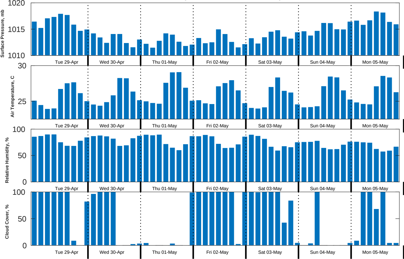
Met Forecast for Brooks McCall from 29-Apr-2025 00:00:00 to 06-May-2025 00:00:00
