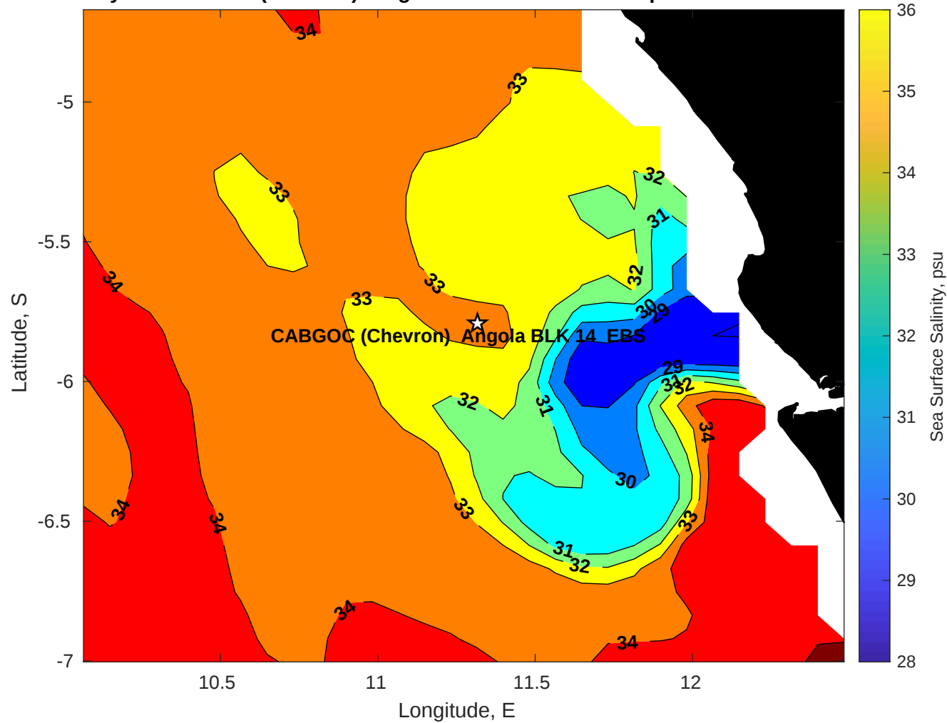
Surface Salinity for CABGOC (Chevron) Angola BLK 14 EBS at 28-Apr-2025 00:00:00
