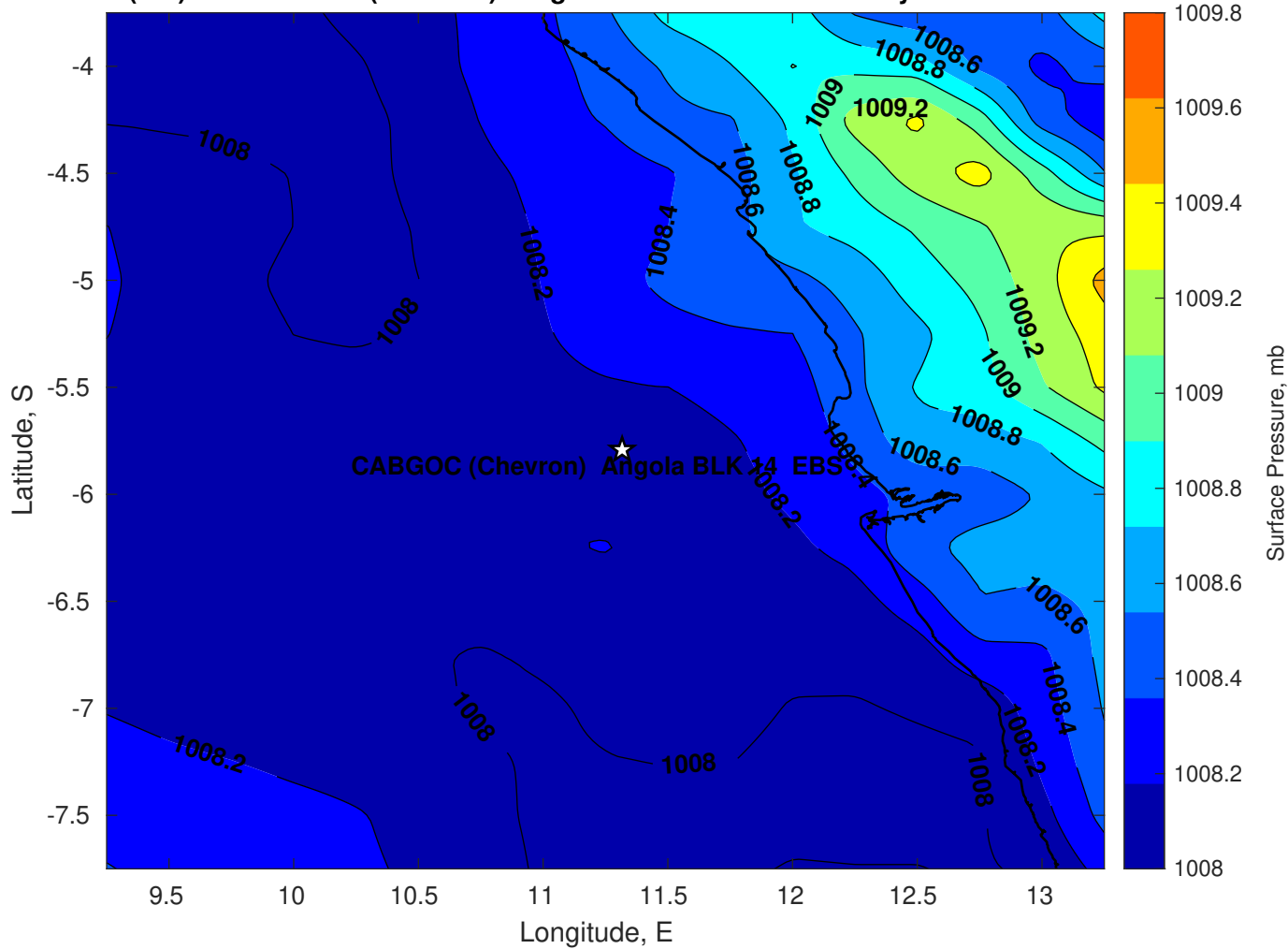
Surface Pressure (mb) for CABGOC (Chevron) Angola BLK 14 EBS at 01-May-2025 00:00:00
