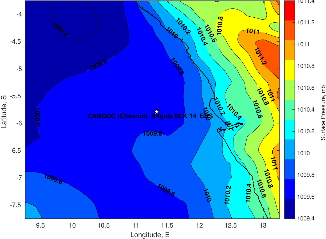
Surface Pressure (mb) for CABGOC (Chevron) Angola BLK 14 EBS at 29-Apr-2025 00:00:00
