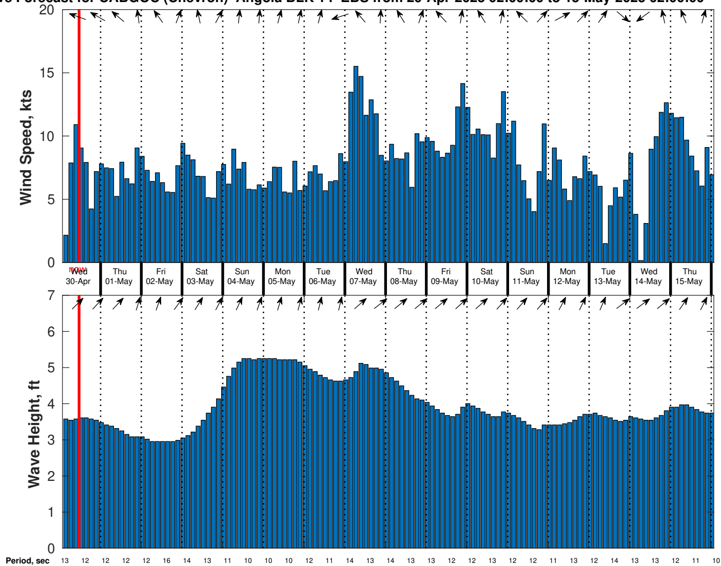
Wind & Wave Forecast for CABGOC (Chevron) Angola BLK 14 EBS from 29-Apr-2025 02:00:00 to 15-May-2025 02:00:00
