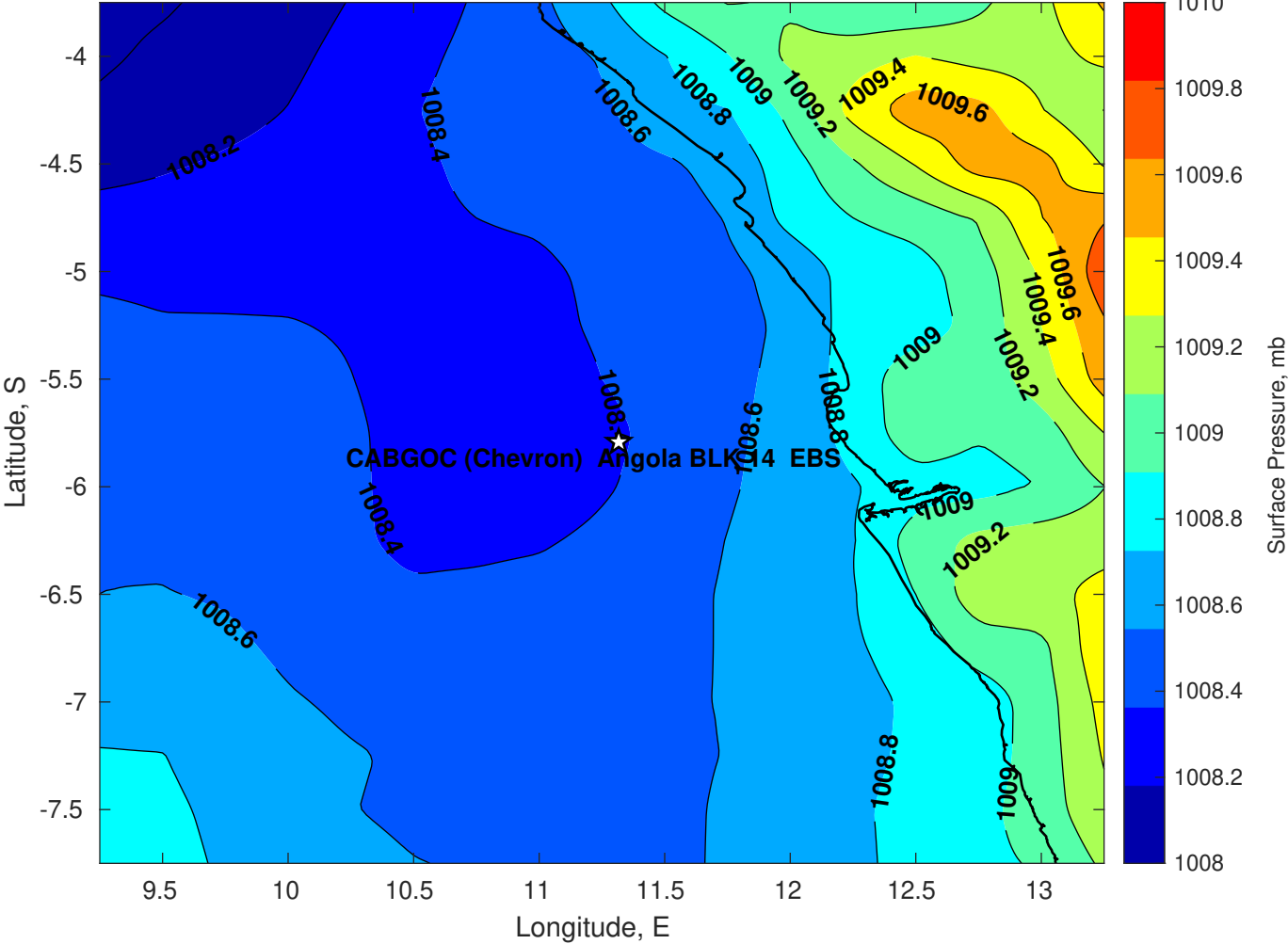
Surface Pressure (mb) for CABGOC (Chevron) Angola BLK 14 EBS at 30-Apr-2025 00:00:00
