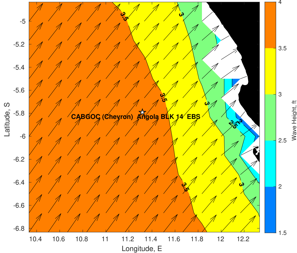
Wave Height (ft) for CABGOC (Chevron) Angola BLK 14 EBS at 29-Apr-2025 09:00:00
