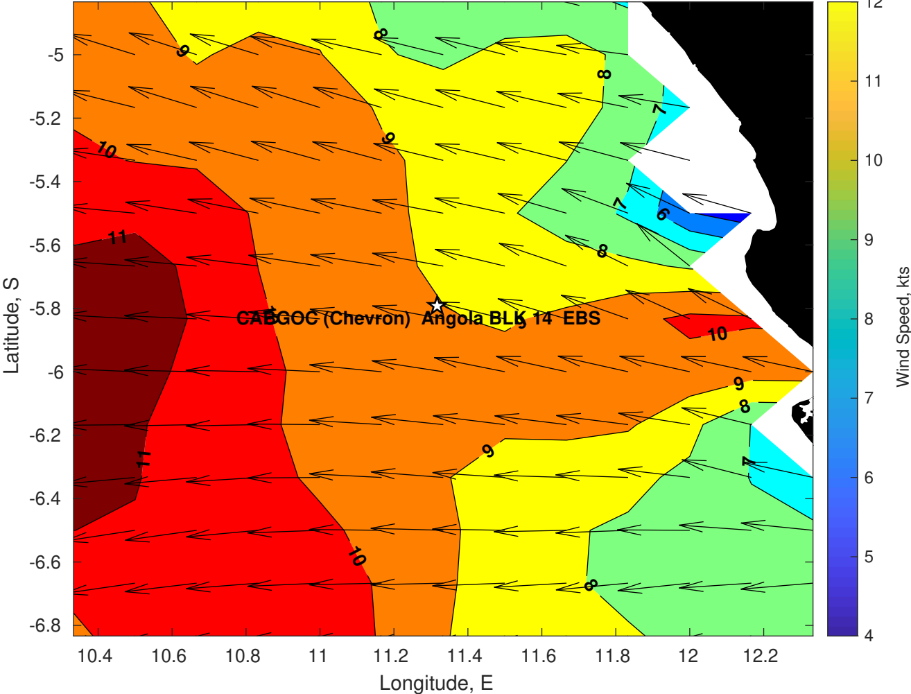
Winds (kts) for CABGOC (Chevron) Angola BLK 14 EBS at 29-Apr-2025 09:00:00
