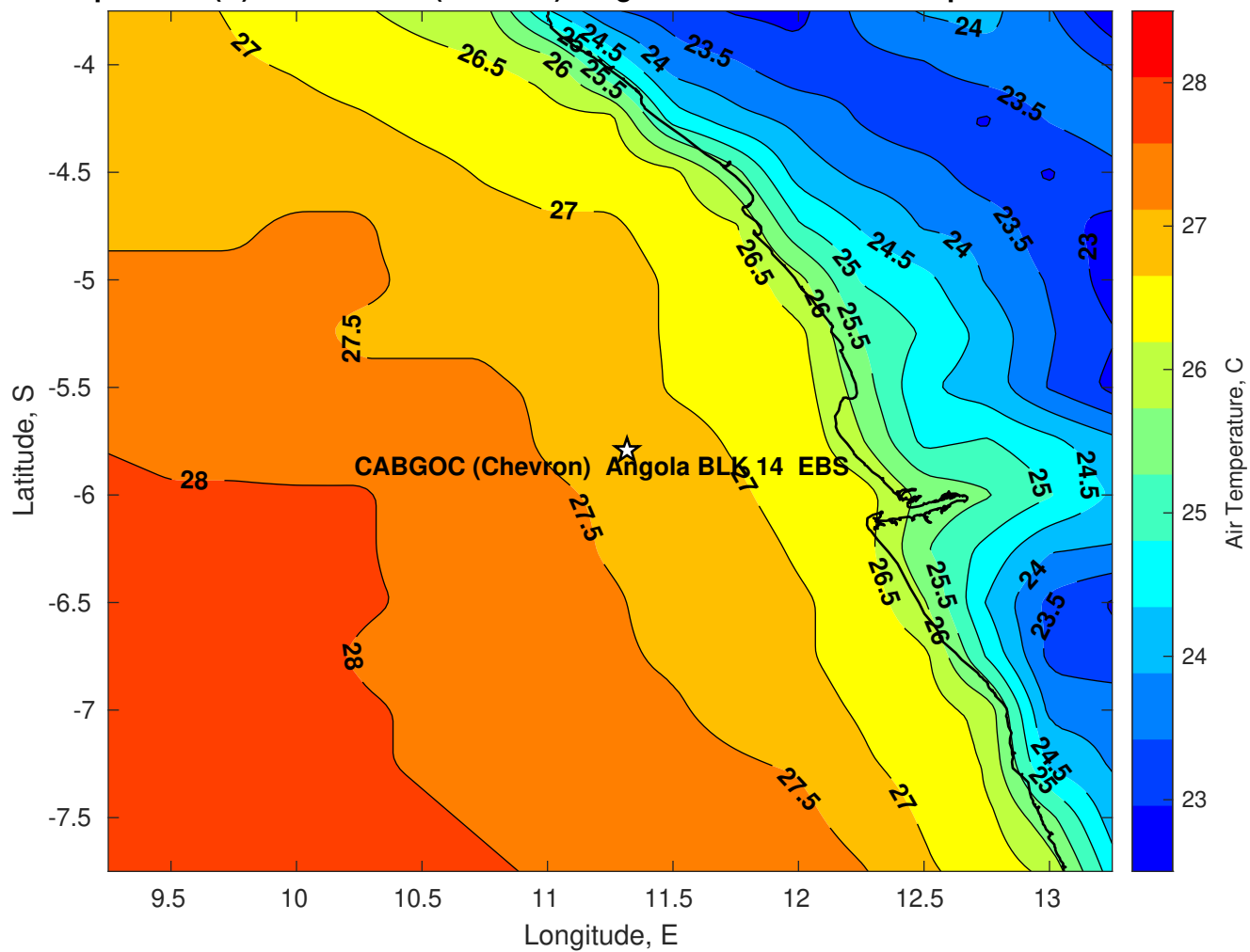
Air Temperature (C) for CABGOC (Chevron) Angola BLK 14 EBS at 29-Apr-2025
