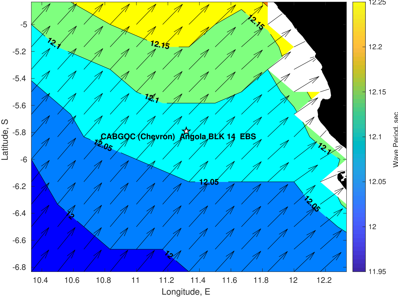
Wave Period (sec) for CABGOC (Chevron) Angola BLK 14 EBS at 29-Apr-2025 09:00:00
