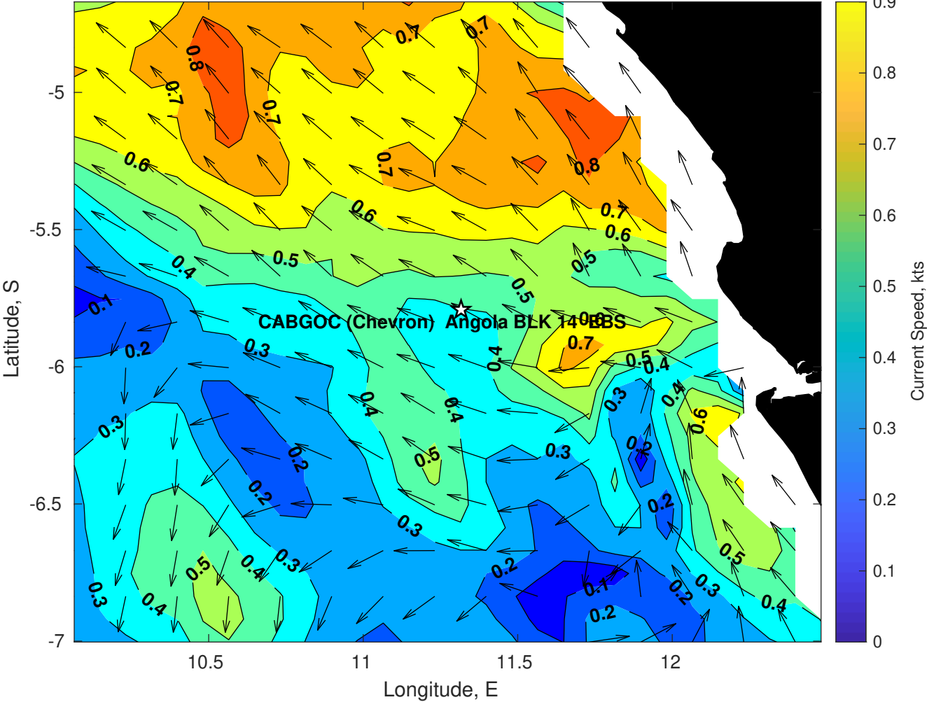
Surface Currents for CABGOC (Chevron) Angola BLK 14 EBS at 28-Apr-2025 00:00:00
