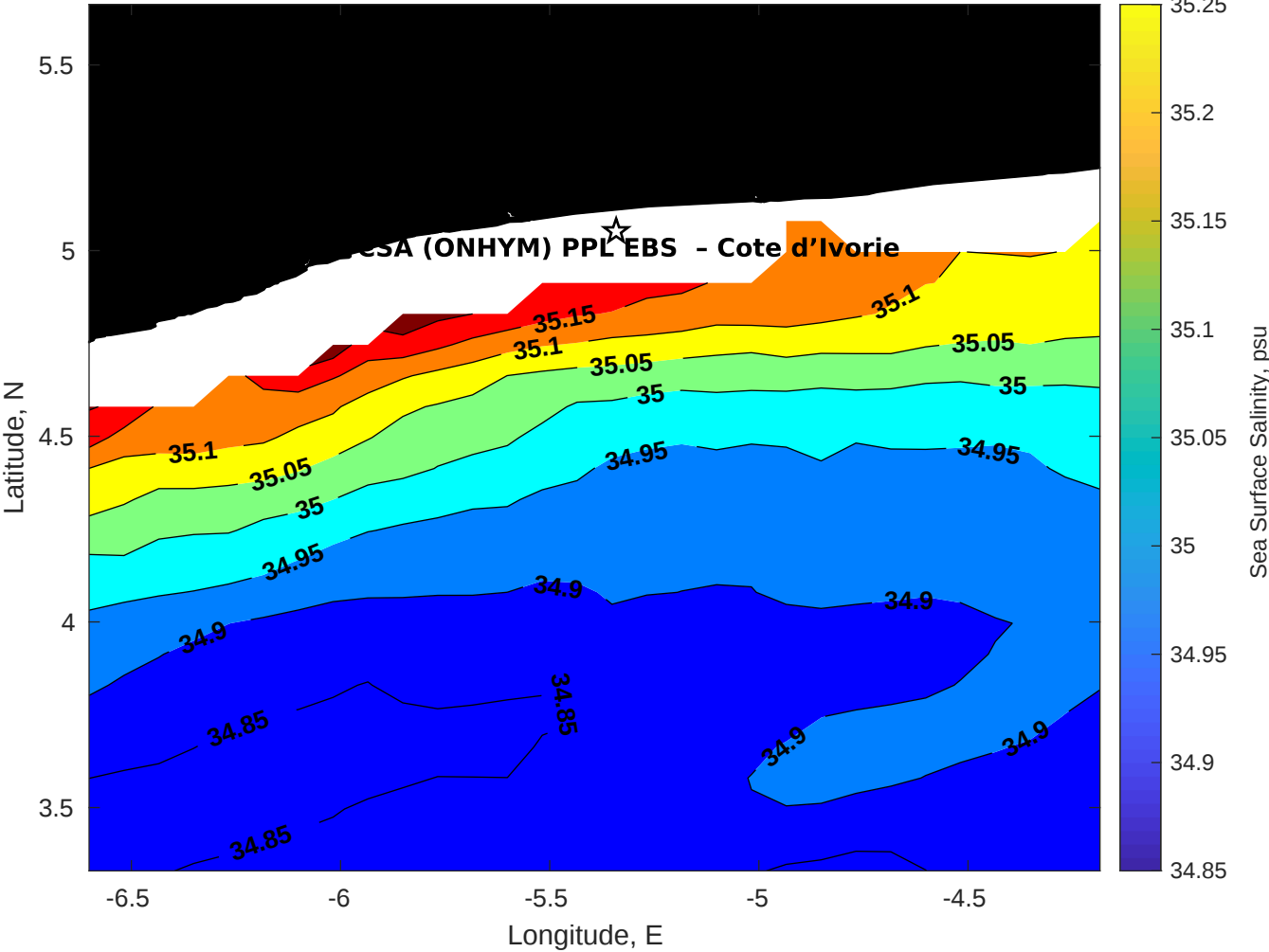
Surface Salinity for CSA (ONHYM) PPL EBS - Cote d'Ivoire at 28-Apr-2025 00:00:00
