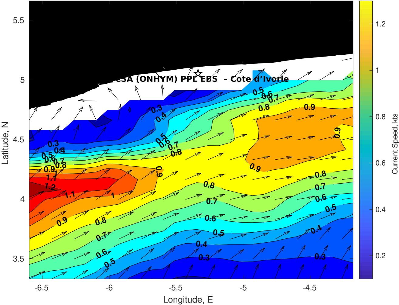
Surface Currents for CSA (ONHYM) PPL EBS - Cote d'Ivoire at 28-Apr-2025 00:00:00
