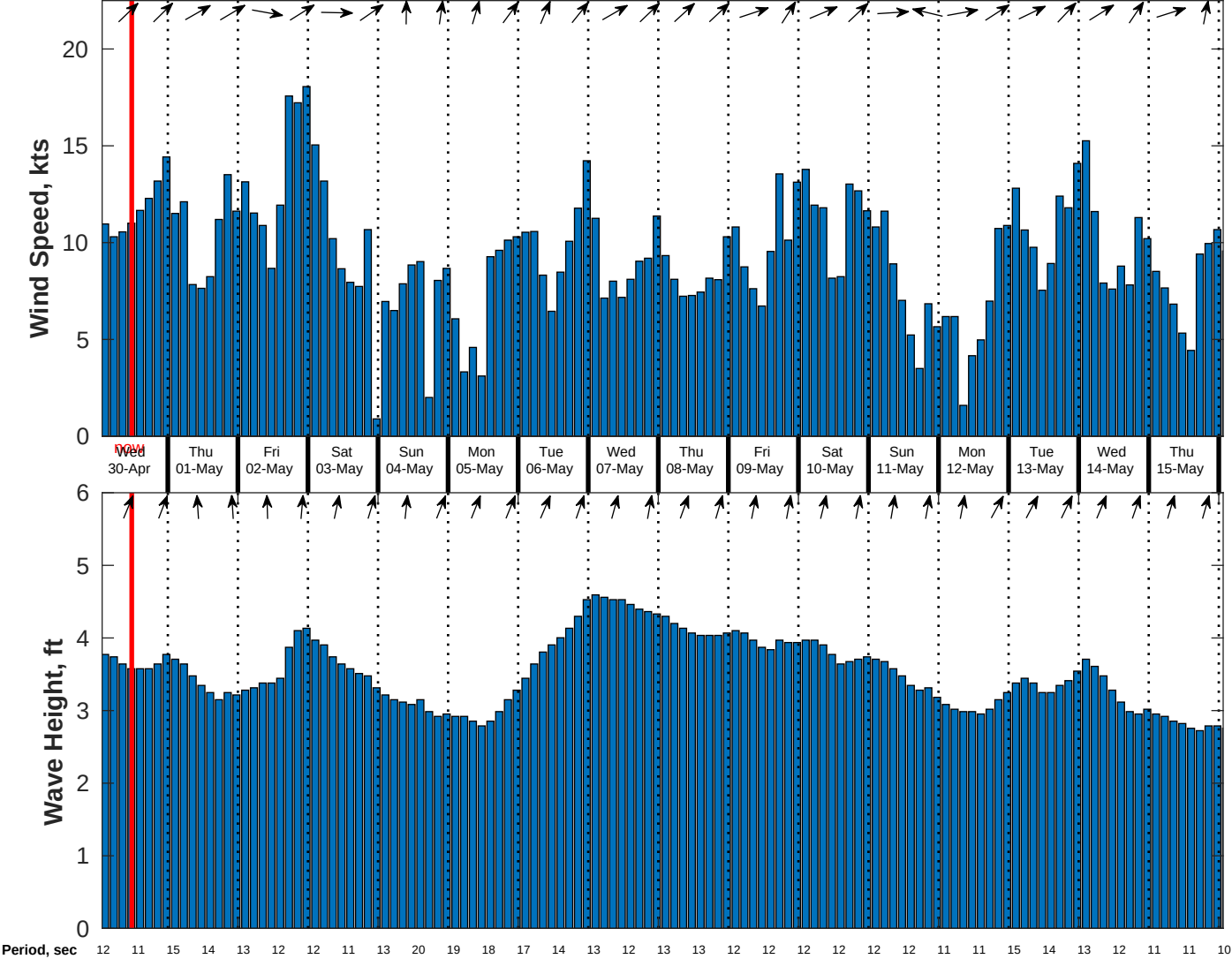
Wind & Wave Forecast for CSA (ONHYM) PPL EBS - Cote d'Ivoire from 29-Apr-2025 01:00:00 to 15-May-2025 01:00:00
