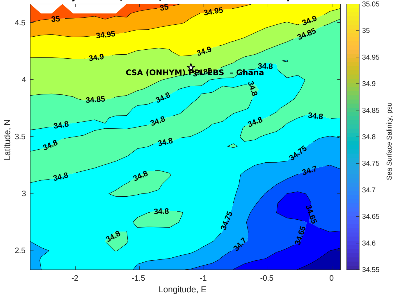
Surface Salinity for CSA (ONHYM) PPL EBS - Ghana at 28-Apr-2025 00:00:00
