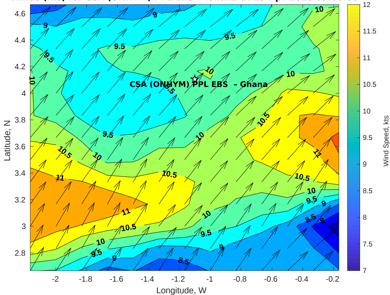
Winds (kts) for CSA (ONHYM) PPL EBS - Ghana at 29-Apr-2025 09:00:00
