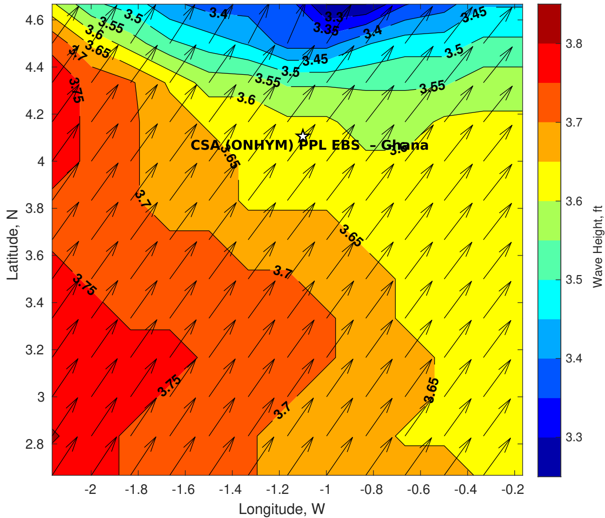
Wave Height (ft) for CSA (ONHYM) PPL EBS - Ghana at 29-Apr-2025 09:00:00
