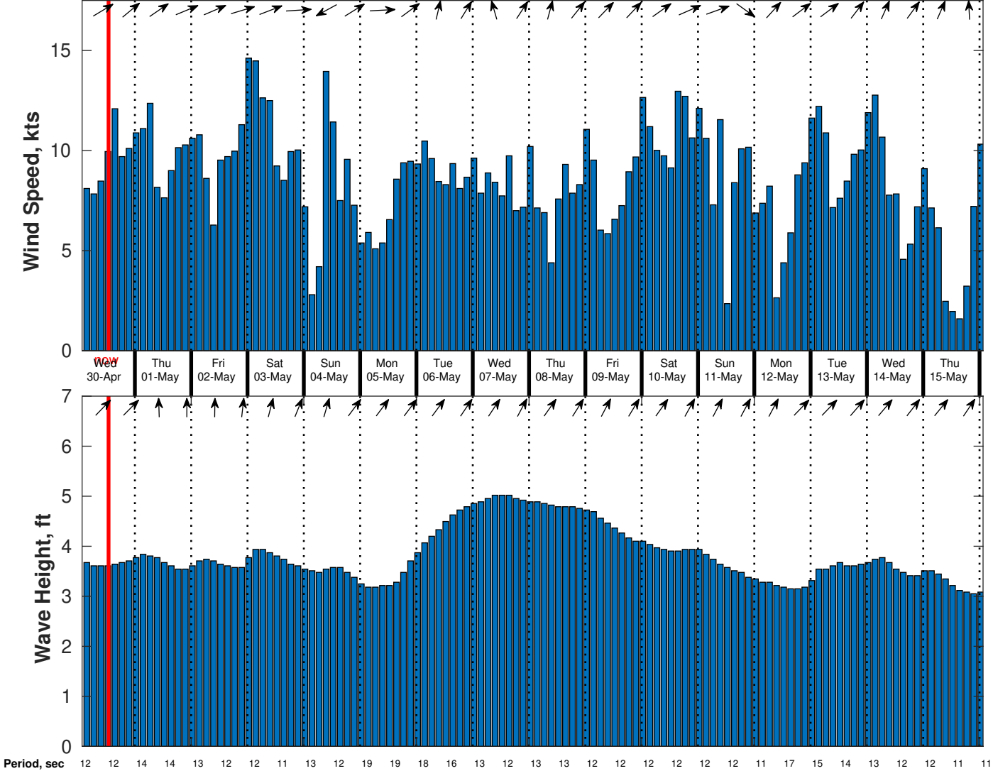
Wind & Wave Forecast for CSA (ONHYM) PPL EBS - Ghana from 29-Apr-2025 02:00:00 to 15-May-2025 02:00:00
