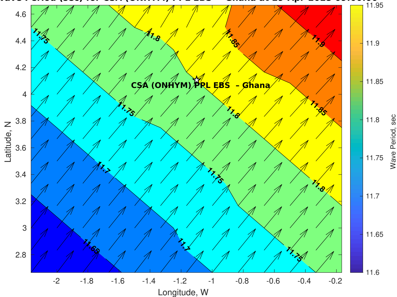
Wave Period (sec) for CSA (ONHYM) PPL EBS - Ghana at 29-Apr-2025 09:00:00
