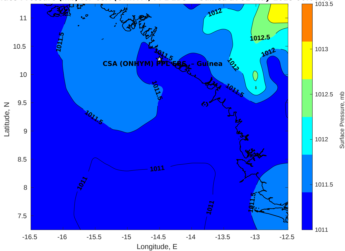
Surface Pressure (mb) for CSA (ONHYM) PPL EBS - Guinea at 01-May-2025 00:00:00
