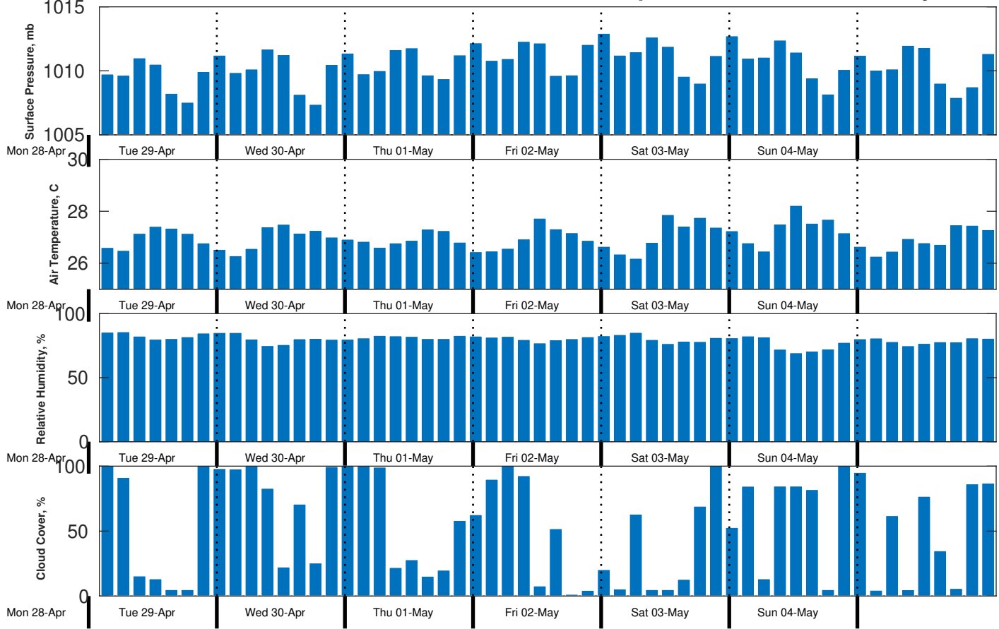
Met Forecast for CSA (ONHYM) PPL EBS - Guinea from 29-Apr-2025 00:00:00 to 06-May-2025 00:00:00
