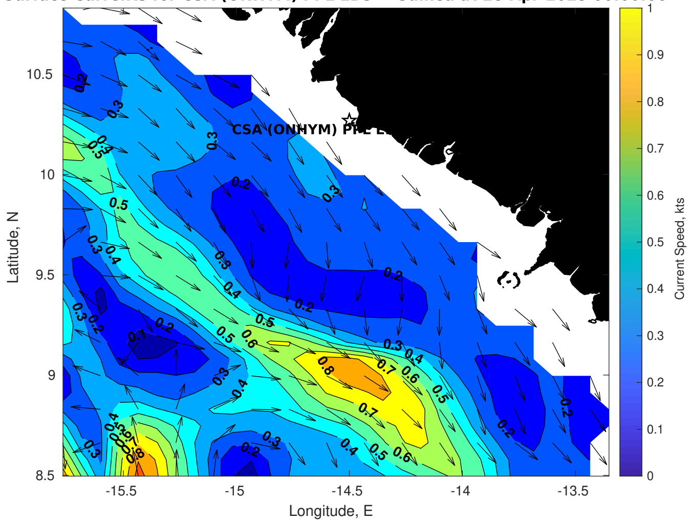
Surface Currents for CSA (ONHYM) PPL EBS - Guinea at 28-Apr-2025 00:00:00
