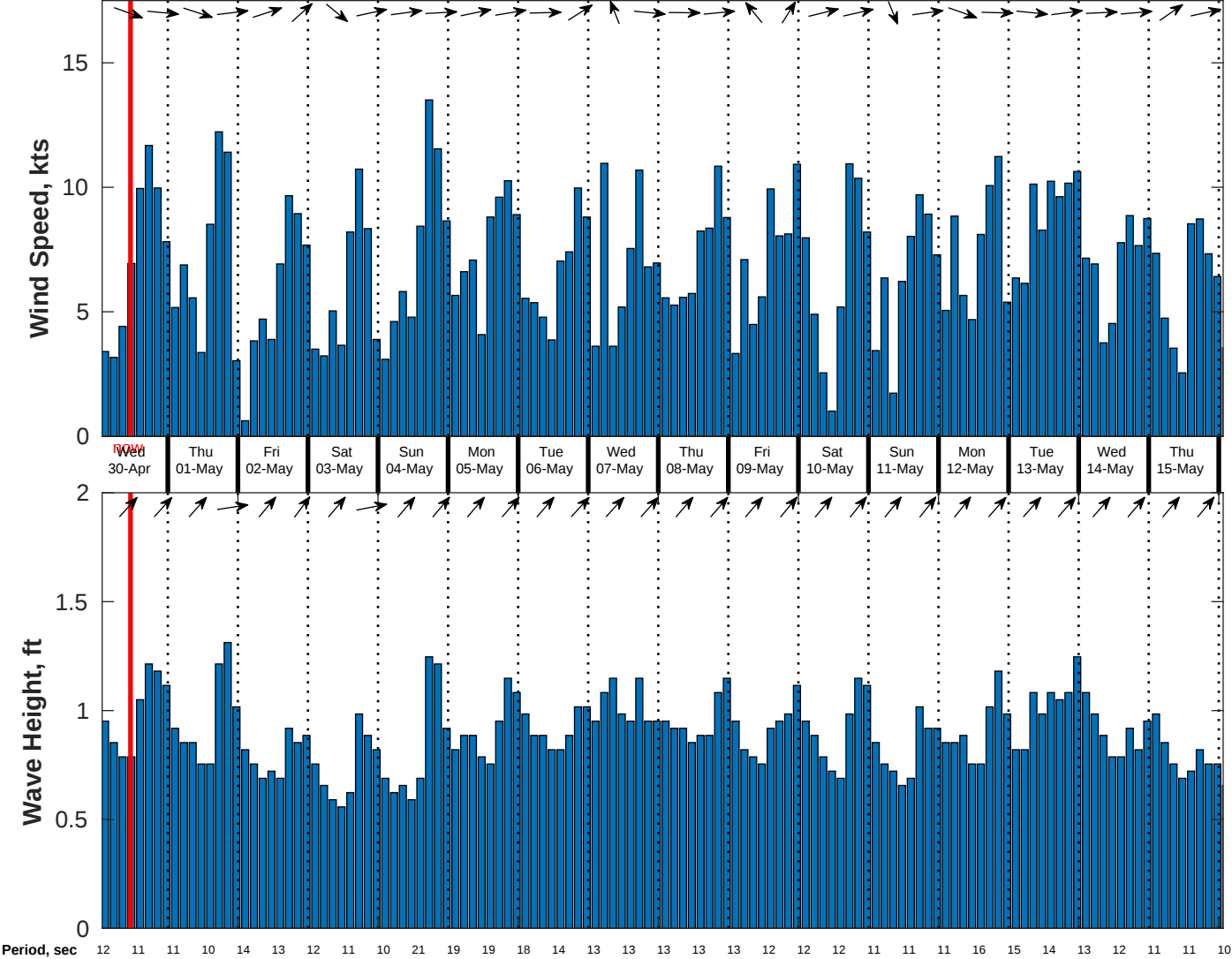
Wind & Wave Forecast for CSA (ONHYM) PPL EBS - Guinea from 29-Apr-2025 01:00:00 to 15-May-2025 01:00:00
