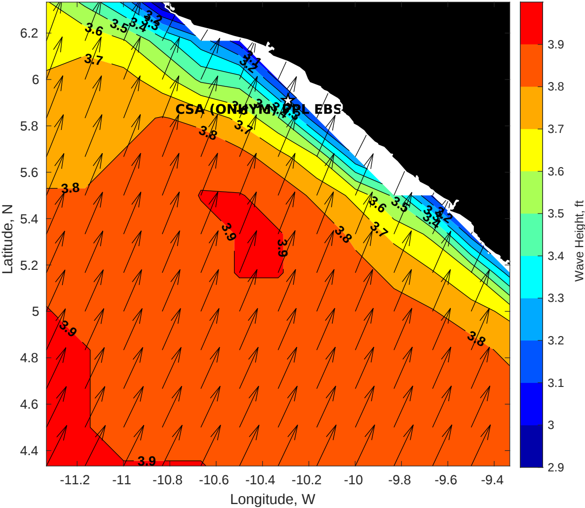
Wave Height (ft) for CSA (ONHYM) PPL EBS - Liberia at 29-Apr-2025 09:00:00
