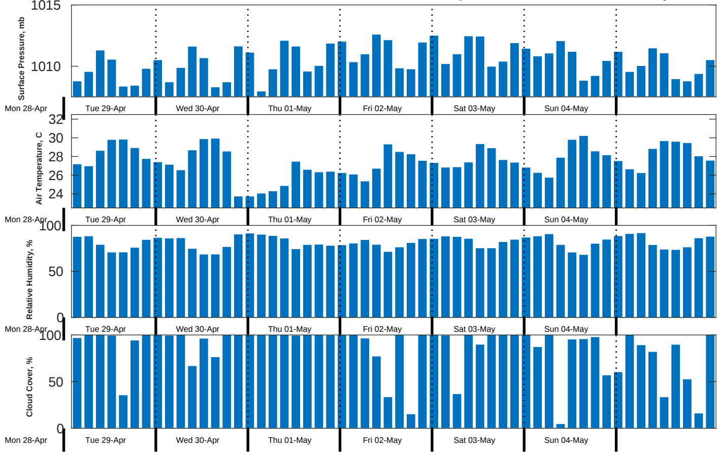
Met Forecast for CSA (ONHYM) PPL EBS - Liberia from 29-Apr-2025 00:00:00 to 06-May-2025 00:00:00
