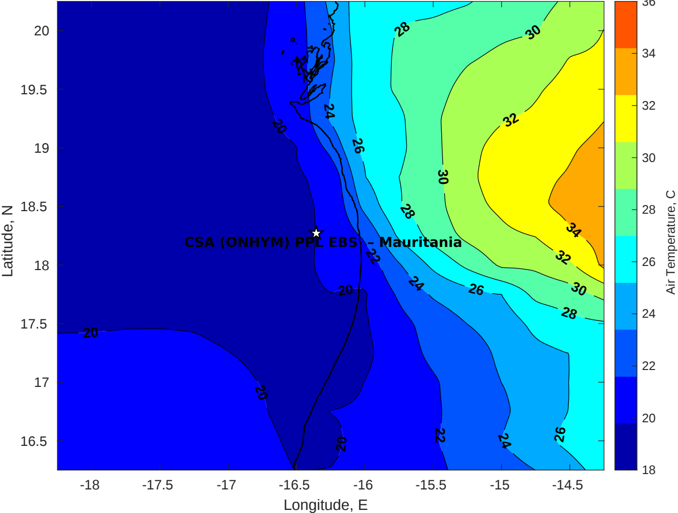
Air Temperature (C) for CSA (ONHYM) PPL EBS - Mauritania at 29-Apr-2025
