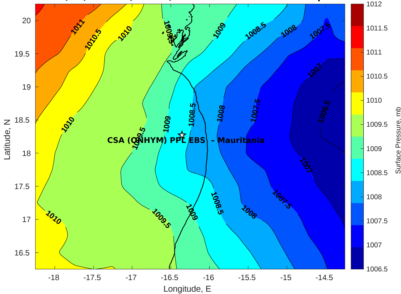
Surface Pressure (mb) for CSA (ONHYM) PPL EBS - Mauritania at 29-Apr-2025 00:00:00
