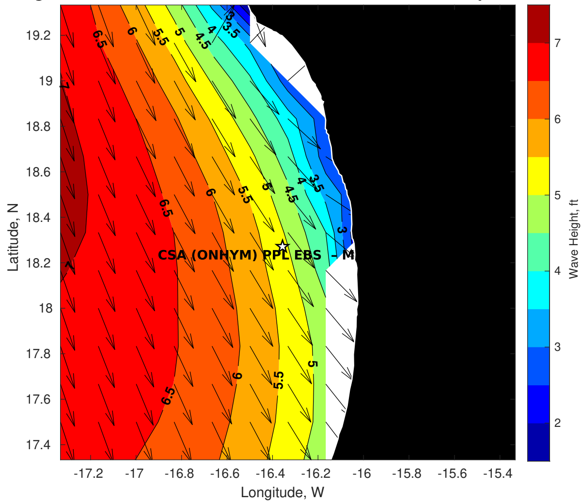
Wave Height (ft) for CSA (ONHYM) PPL EBS - Mauritania at 29-Apr-2025 09:00:00
