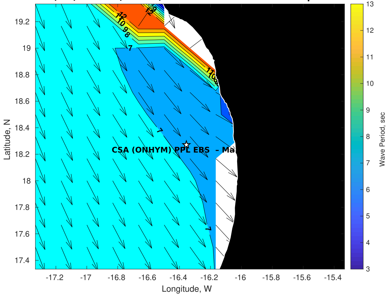
Wave Period (sec) for CSA (ONHYM) PPL EBS - Mauritania at 29-Apr-2025 09:00:00
