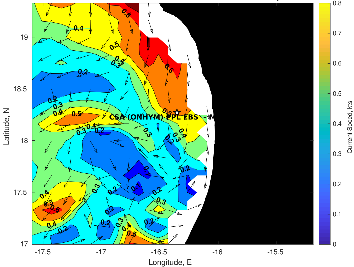
Surface Currents for CSA (ONHYM) PPL EBS - Mauritania at 28-Apr-2025 00:00:00
