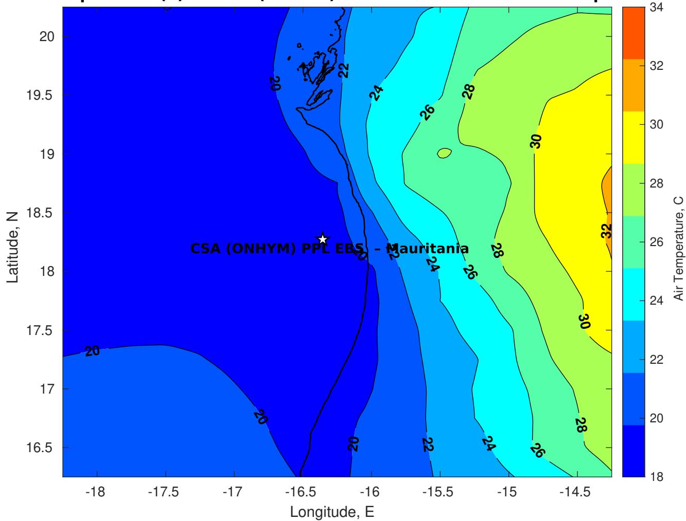
Air Temperature (C) for CSA (ONHYM) PPL EBS - Mauritania at 29-Apr-2025
