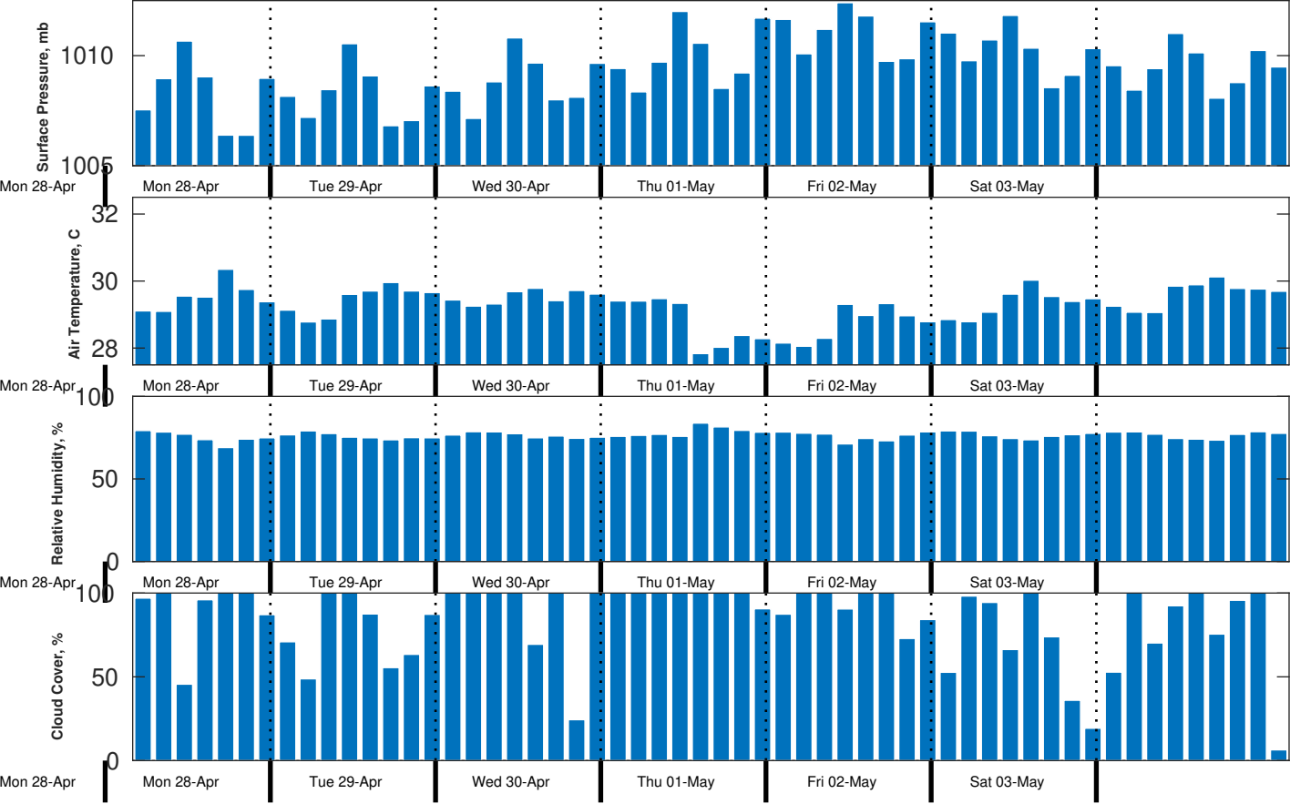
Met Forecast for CSA (ONHYM) PPL EBS - Nigeria from 29-Apr-2025 00:00:00 to 06-May-2025 00:00:00
