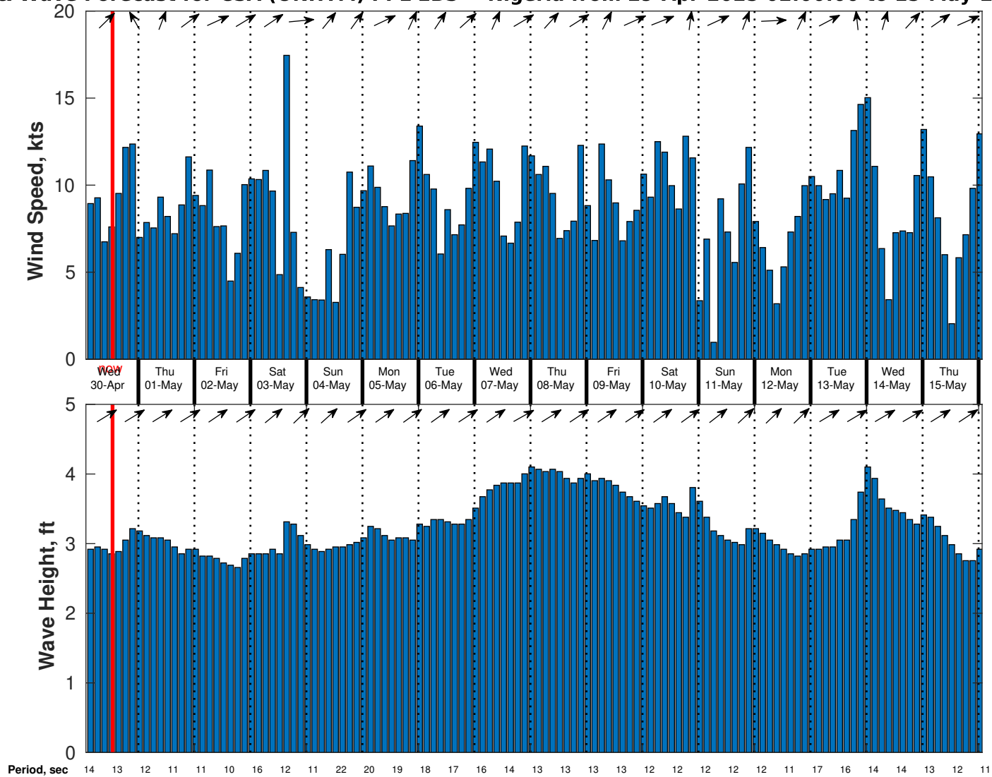
Wind & Wave Forecast for CSA (ONHYM) PPL EBS - Nigeria from 29-Apr-2025 02:00:00 to 15-May-2025 02:00:00
