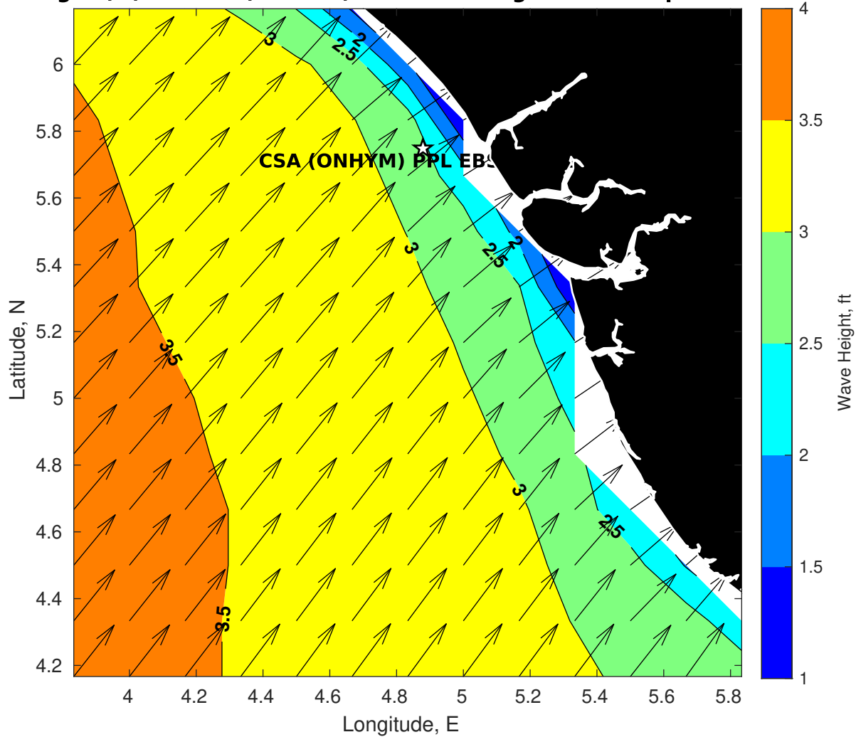
Wave Height (ft) for CSA (ONHYM) PPL EBS - Nigeria at 29-Apr-2025 09:00:00
