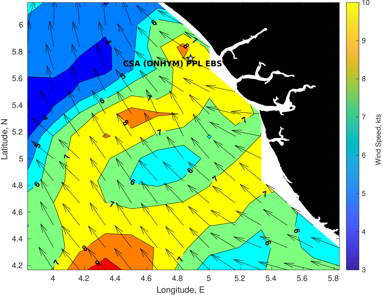
Winds (kts) for CSA (ONHYM) PPL EBS - Nigeria at 29-Apr-2025 09:00:00
