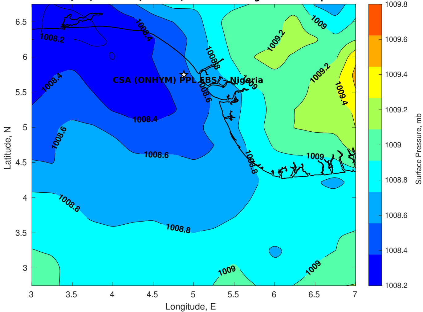
Surface Pressure (mb) for CSA (ONHYM) PPL EBS - Nigeria at 29-Apr-2025 00:00:00
