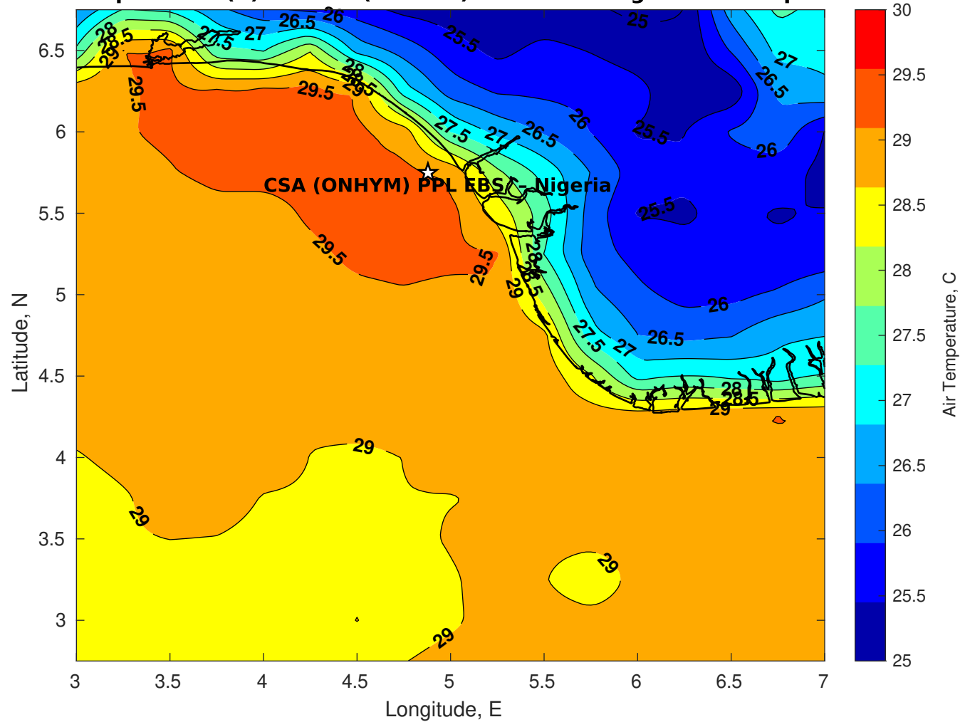
Air Temperature (C) for CSA (ONHYM) PPL EBS - Nigeria at 29-Apr-2025
