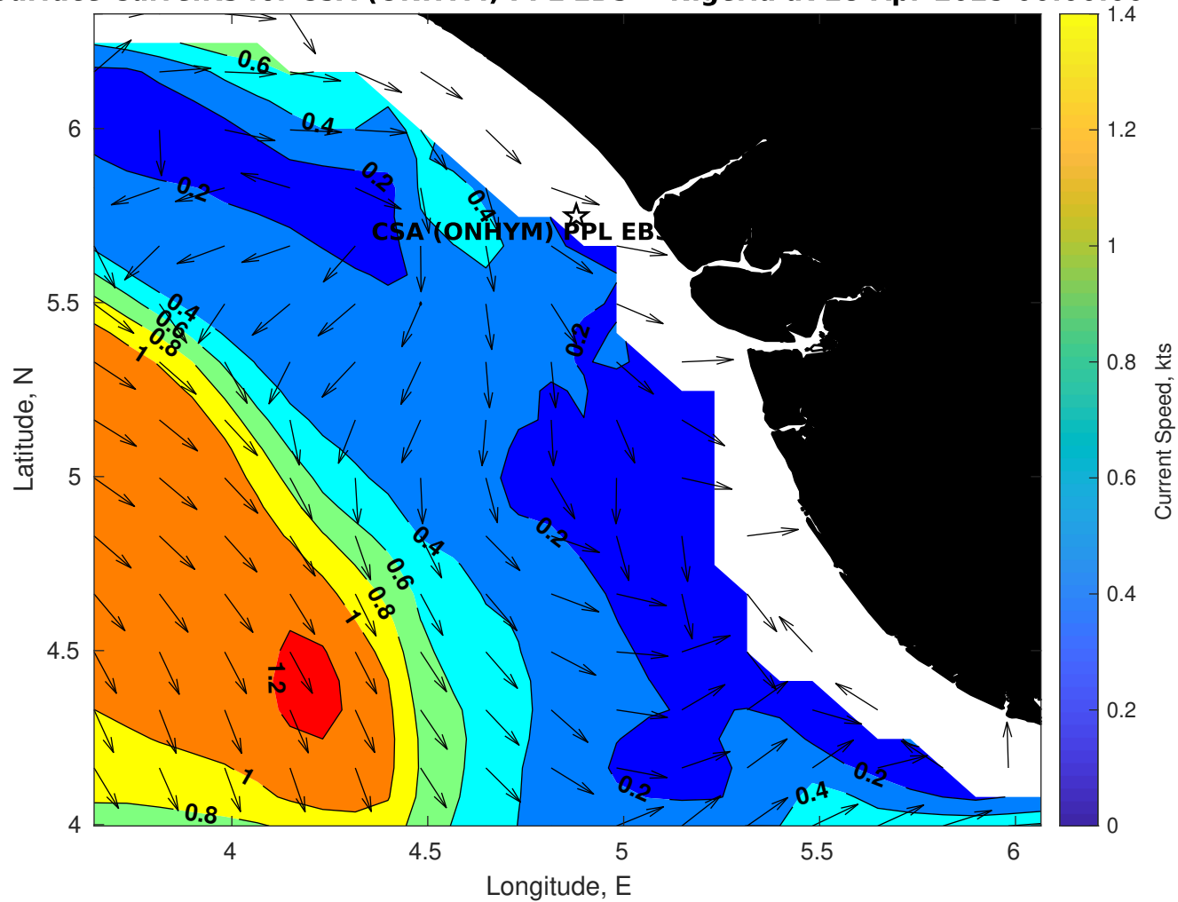
Surface Currents for CSA (ONHYM) PPL EBS - Nigeria at 28-Apr-2025 00:00:00
