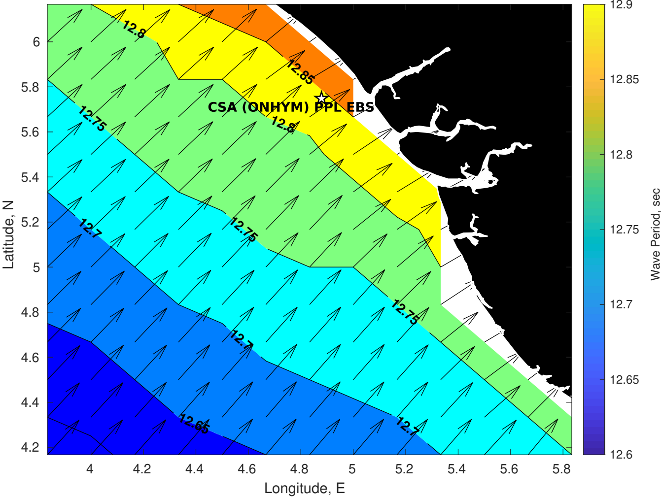
Wave Period (sec) for CSA (ONHYM) PPL EBS - Nigeria at 29-Apr-2025 09:00:00
