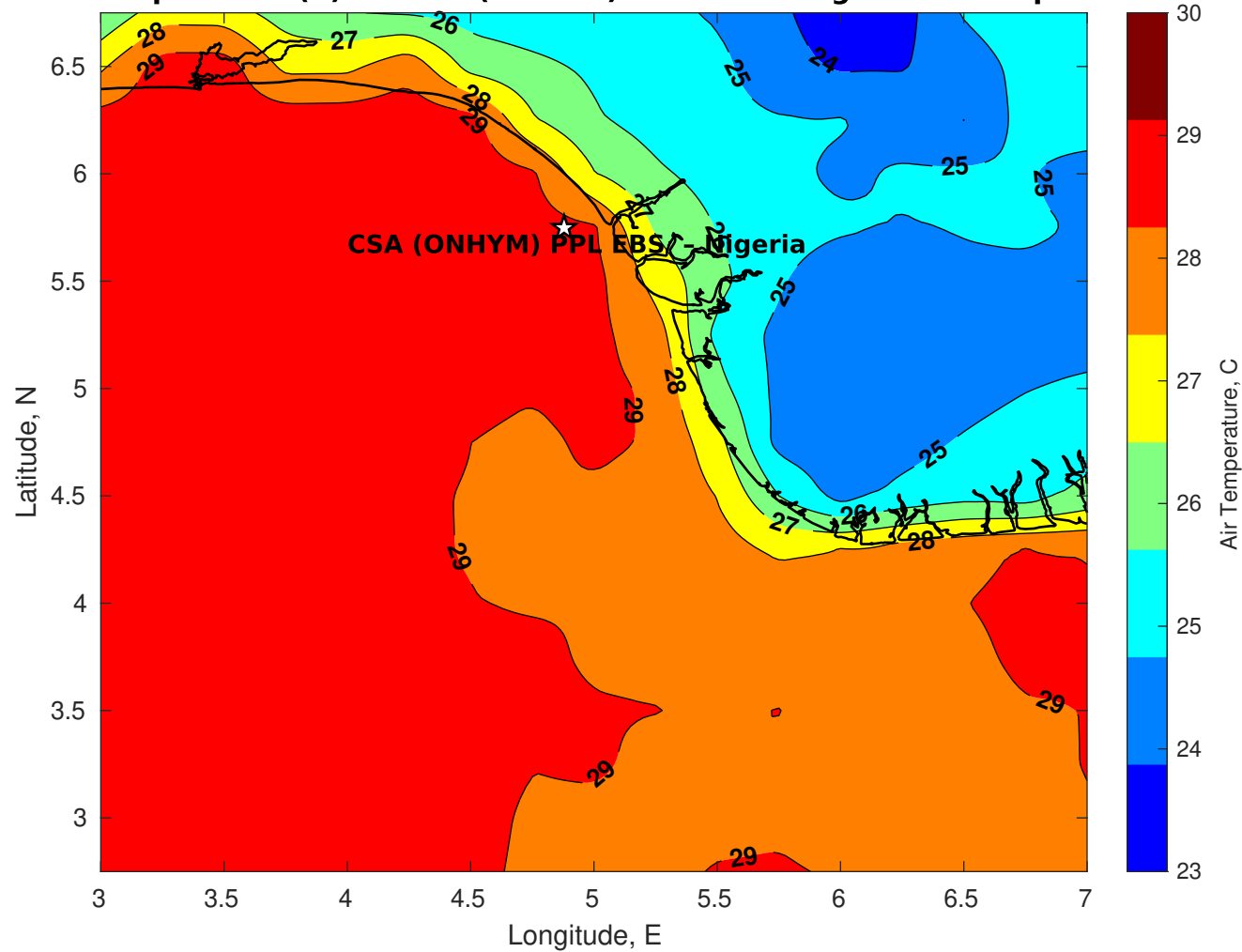
Air Temperature (C) for CSA (ONHYM) PPL EBS - Nigeria at 29-Apr-2025
