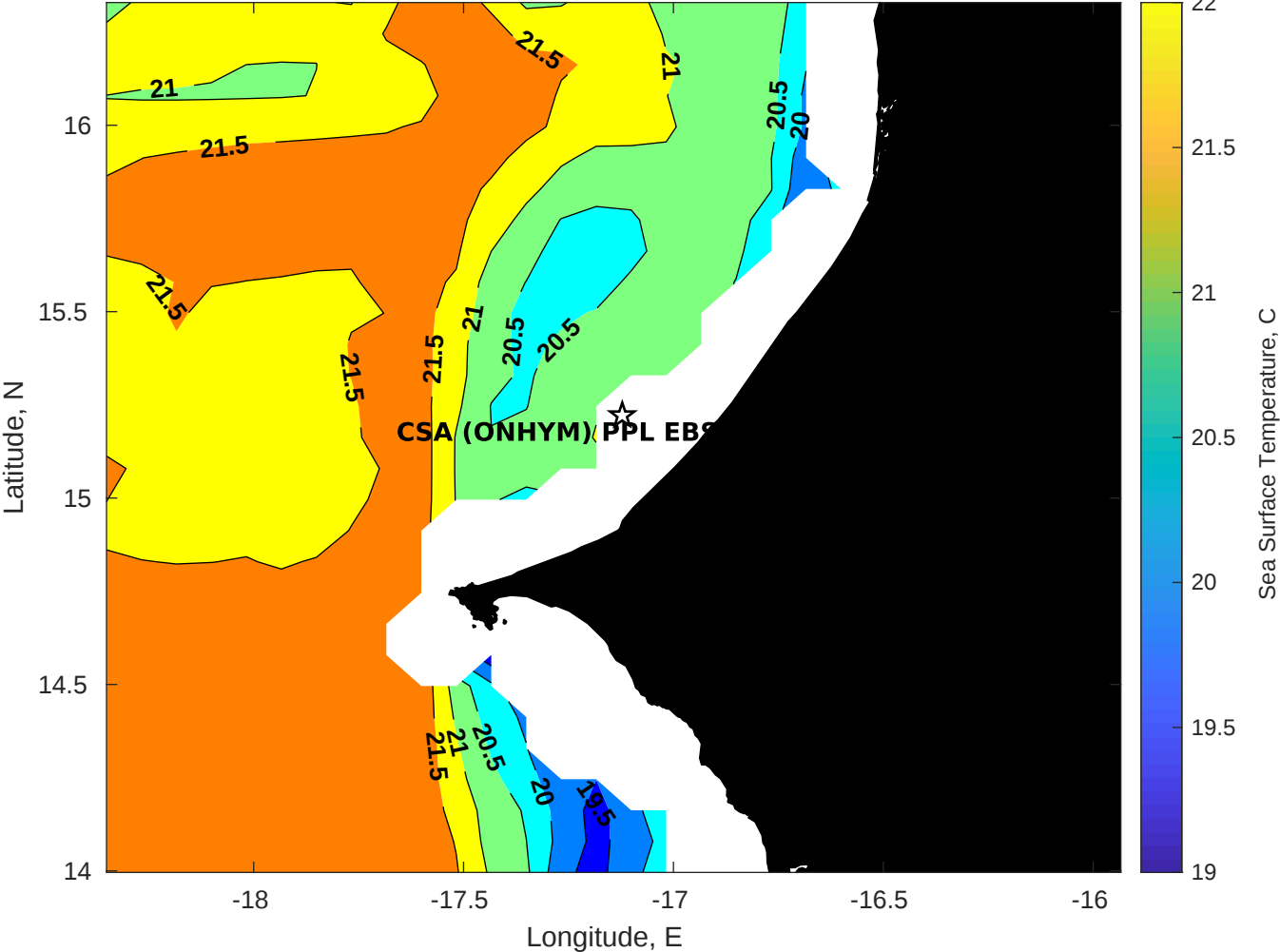
SST for CSA (ONHYM) PPL EBS - Senegal at 28-Apr-2025 00:00:00
