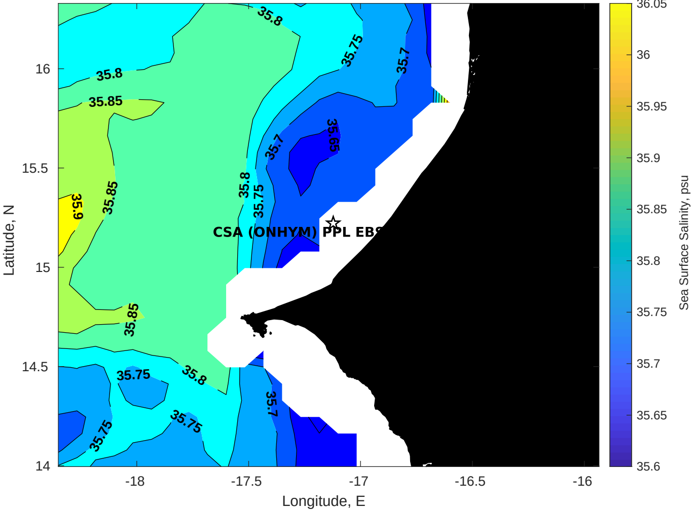
Surface Salinity for CSA (ONHYM) PPL EBS - Senegal at 28-Apr-2025 00:00:00
