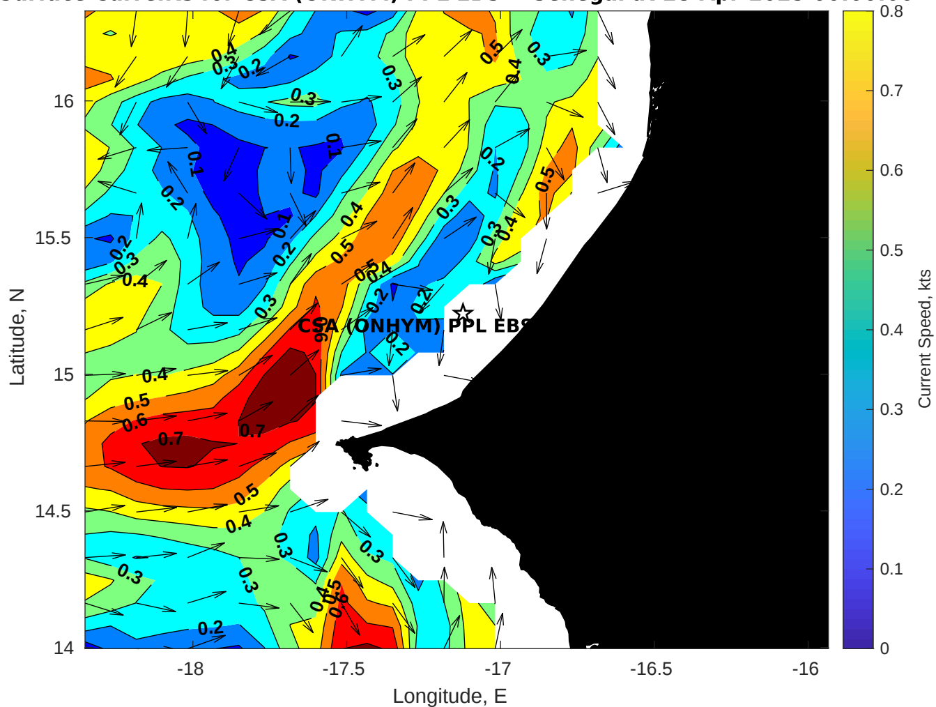
Surface Currents for CSA (ONHYM) PPL EBS - Senegal at 28-Apr-2025 00:00:00
