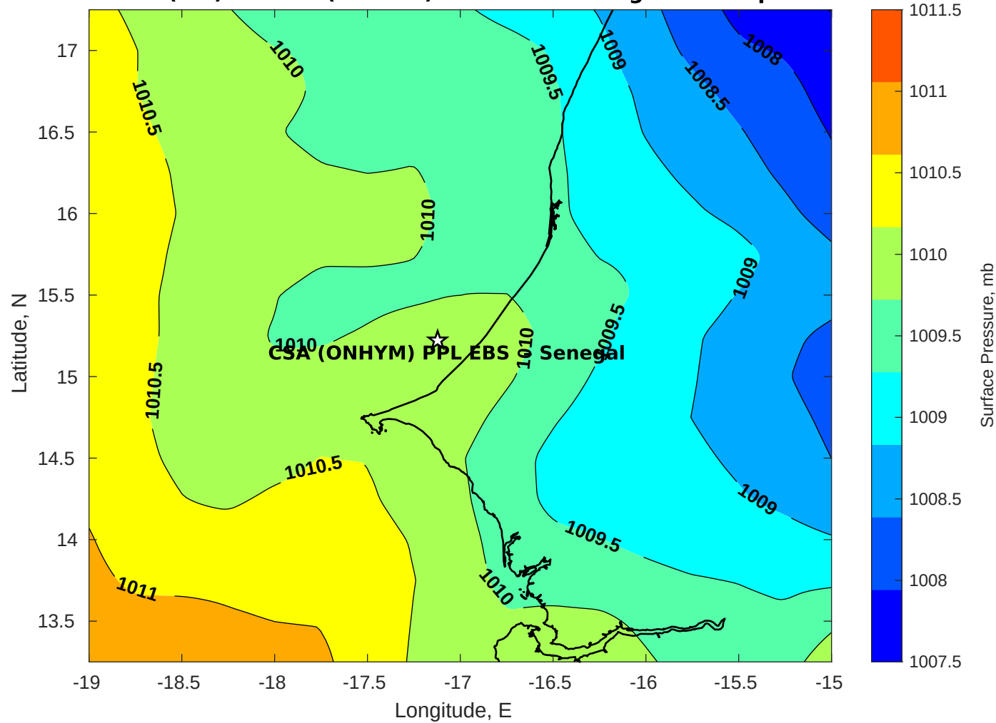
Surface Pressure (mb) for CSA (ONHYM) PPL EBS - Senegal at 29-Apr-2025 00:00:00
