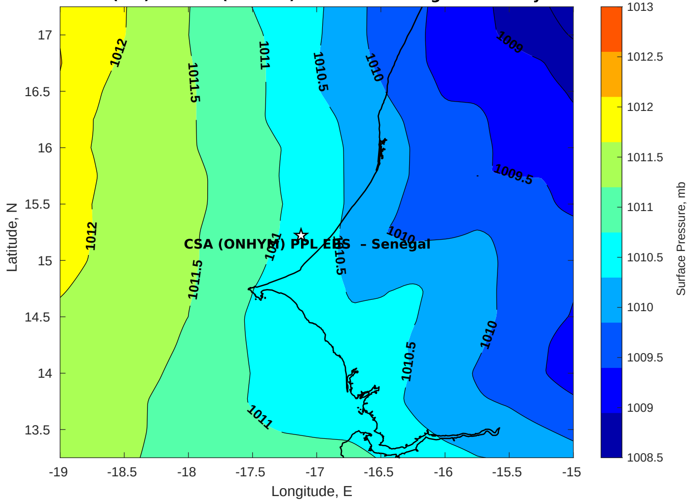
Surface Pressure (mb) for CSA (ONHYM) PPL EBS - Senegal at 01-May-2025 00:00:00
