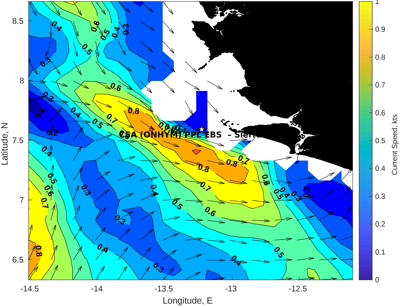
Surface Currents for CSA (ONHYM) PPL EBS - Sierra Leone at 28-Apr-2025 00:00:00
