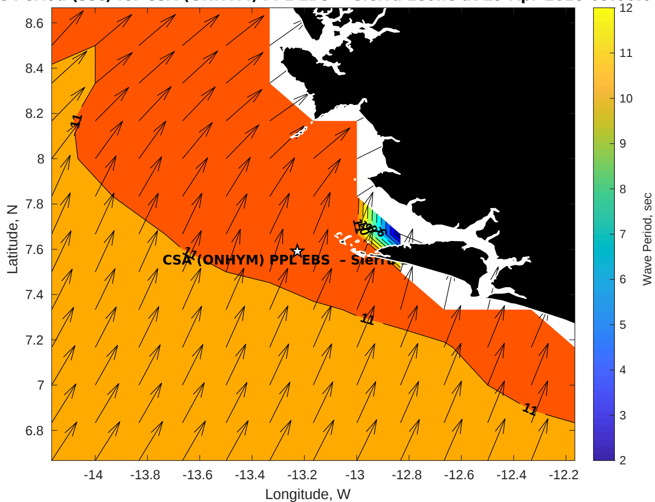
Wave Period (sec) for CSA (ONHYM) PPL EBS - Sierra Leone at 29-Apr-2025 09:00:00
