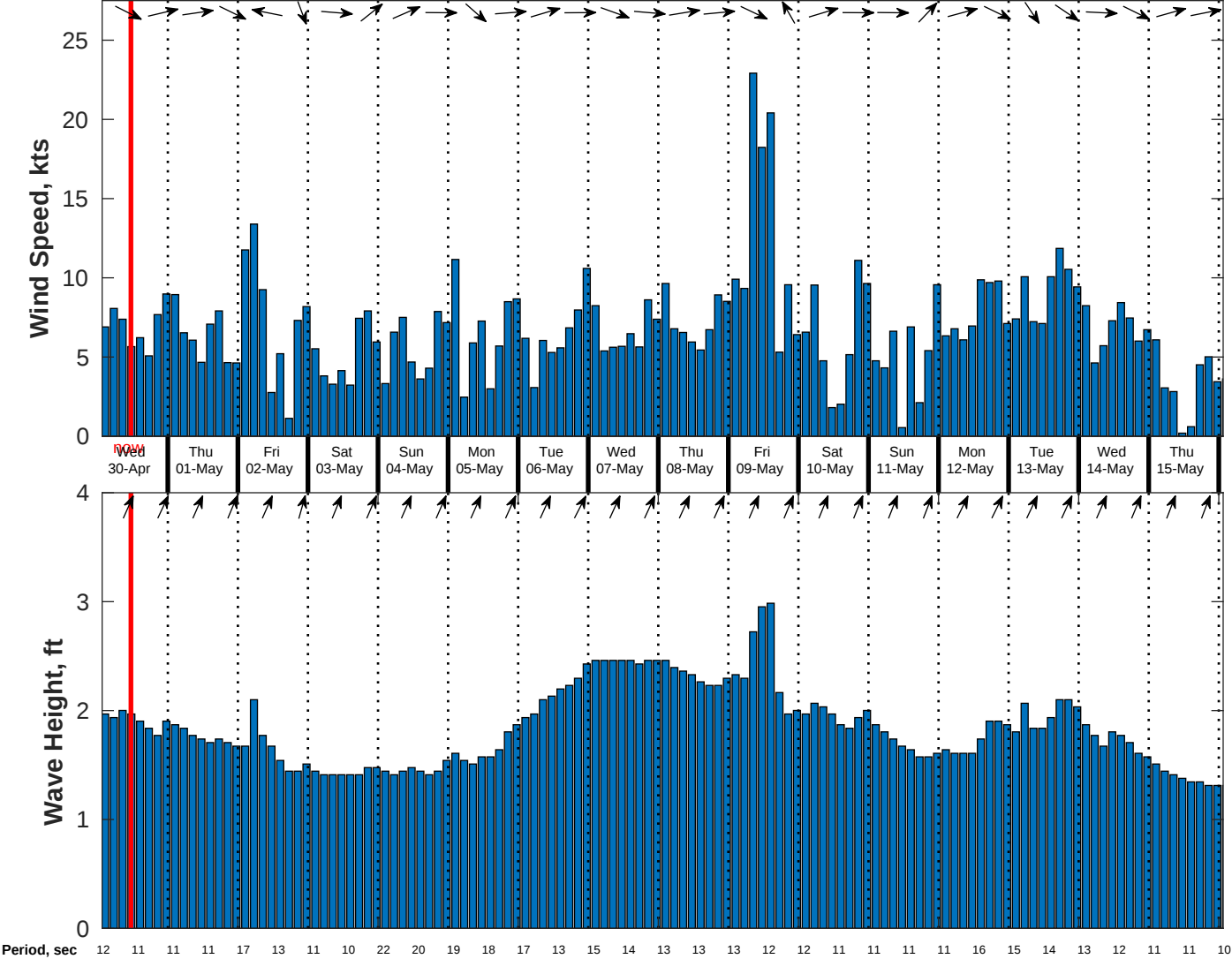
Wind & Wave Forecast for CSA (ONHYM) PPL EBS - Sierra Leone from 29-Apr-2025 01:00:00 to 15-May-2025 01:00:00
