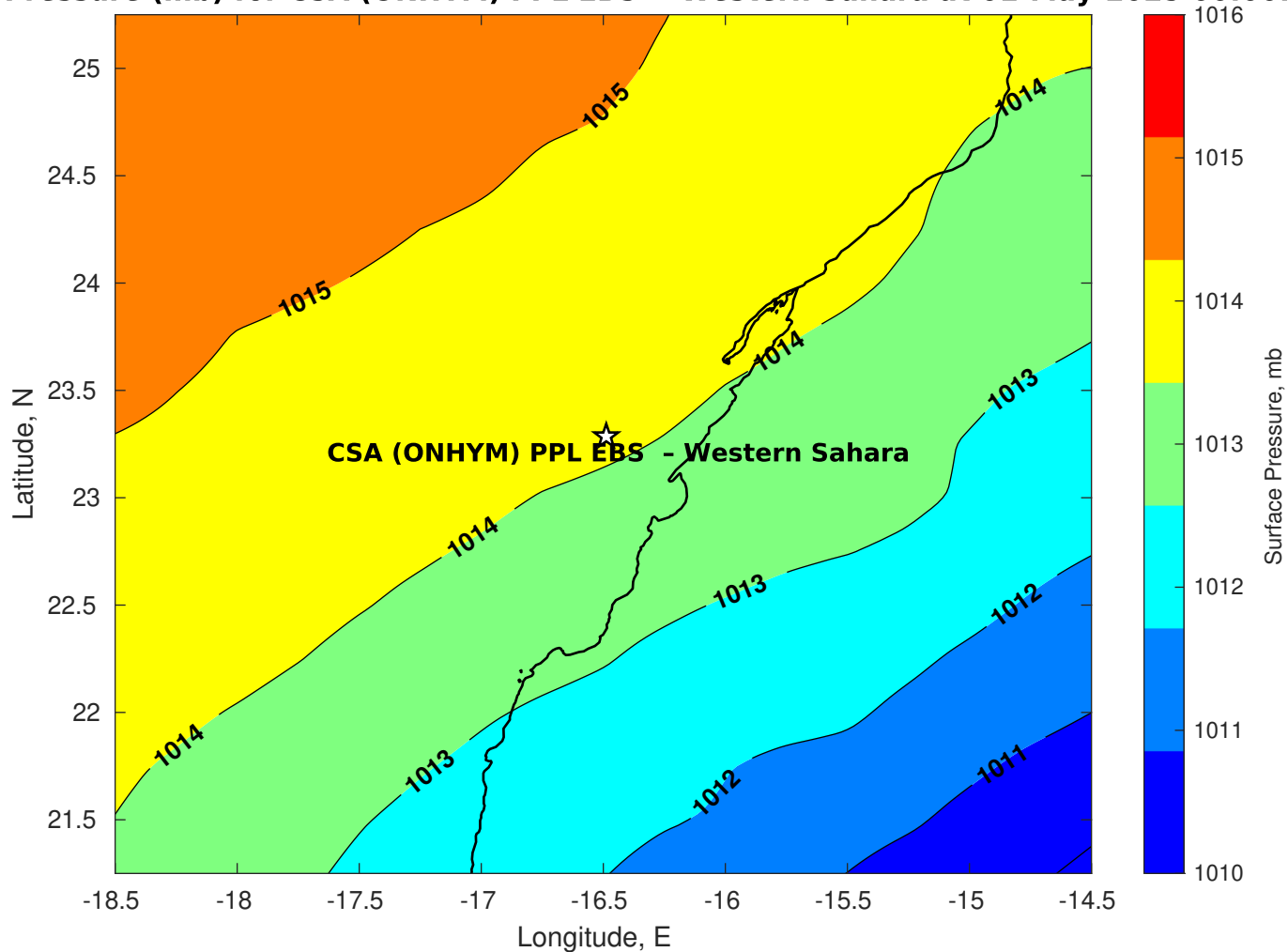
Surface Pressure (mb) for CSA (ONHYM) PPL EBS - Western Sahara at 01-May-2025 00:00:00
