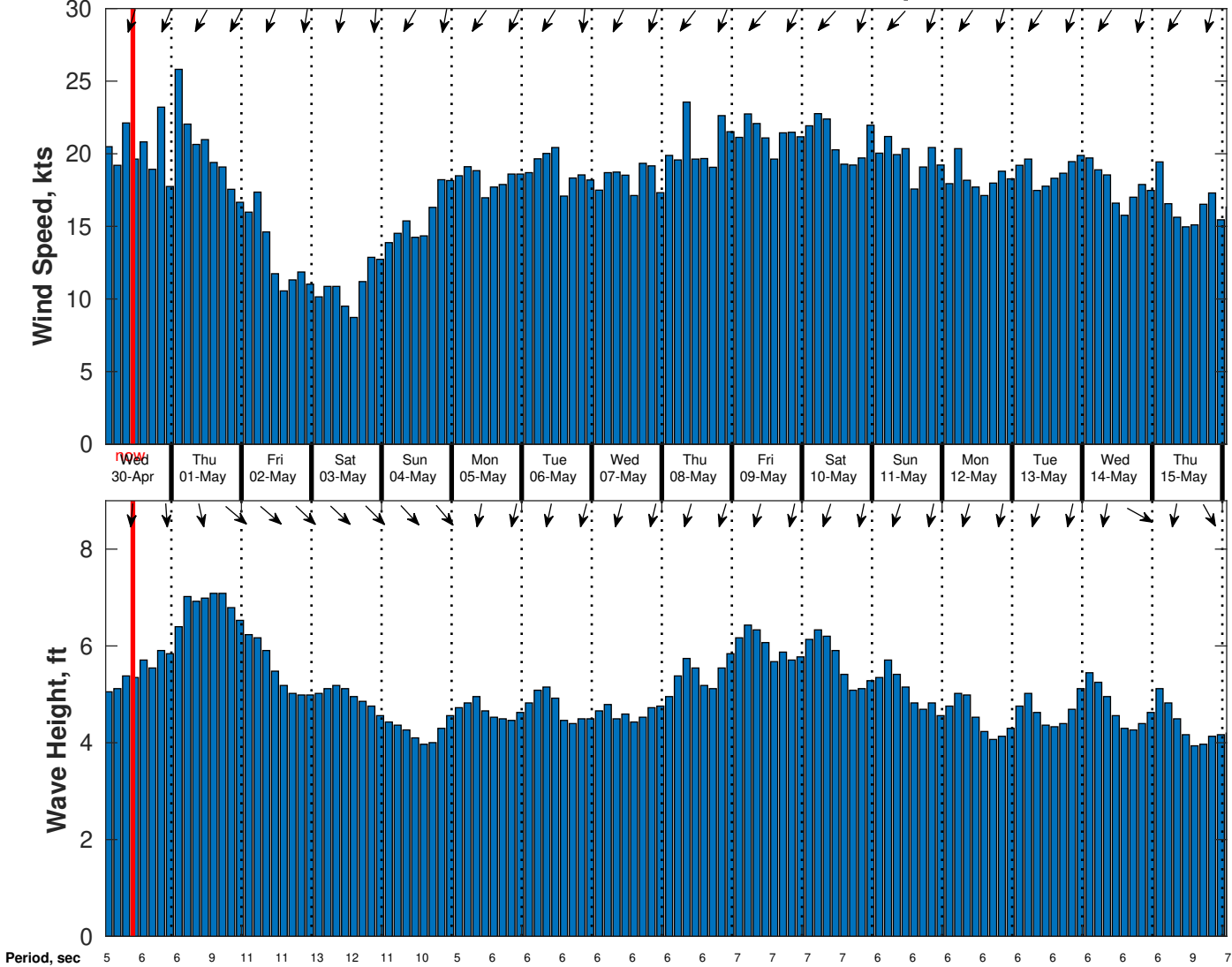
Wind & Wave Forecast for CSA (ONHYM) PPL EBS - Western Sahara from 29-Apr-2025 01:00:00 to 15-May-2025 01:00:00
