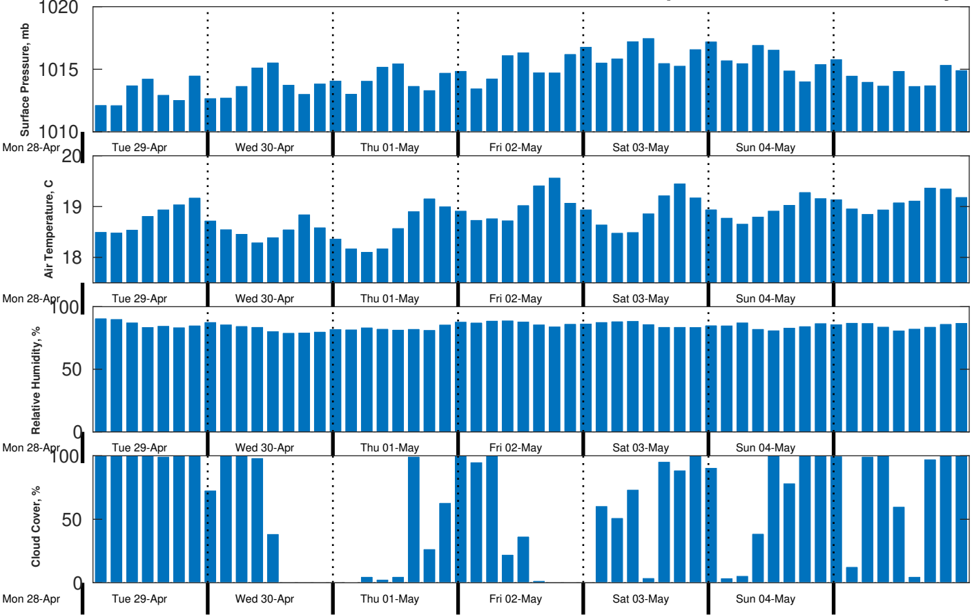
Met Forecast for CSA (ONHYM) PPL EBS - Western Sahara from 29-Apr-2025 00:00:00 to 06-May-2025 00:00:00
