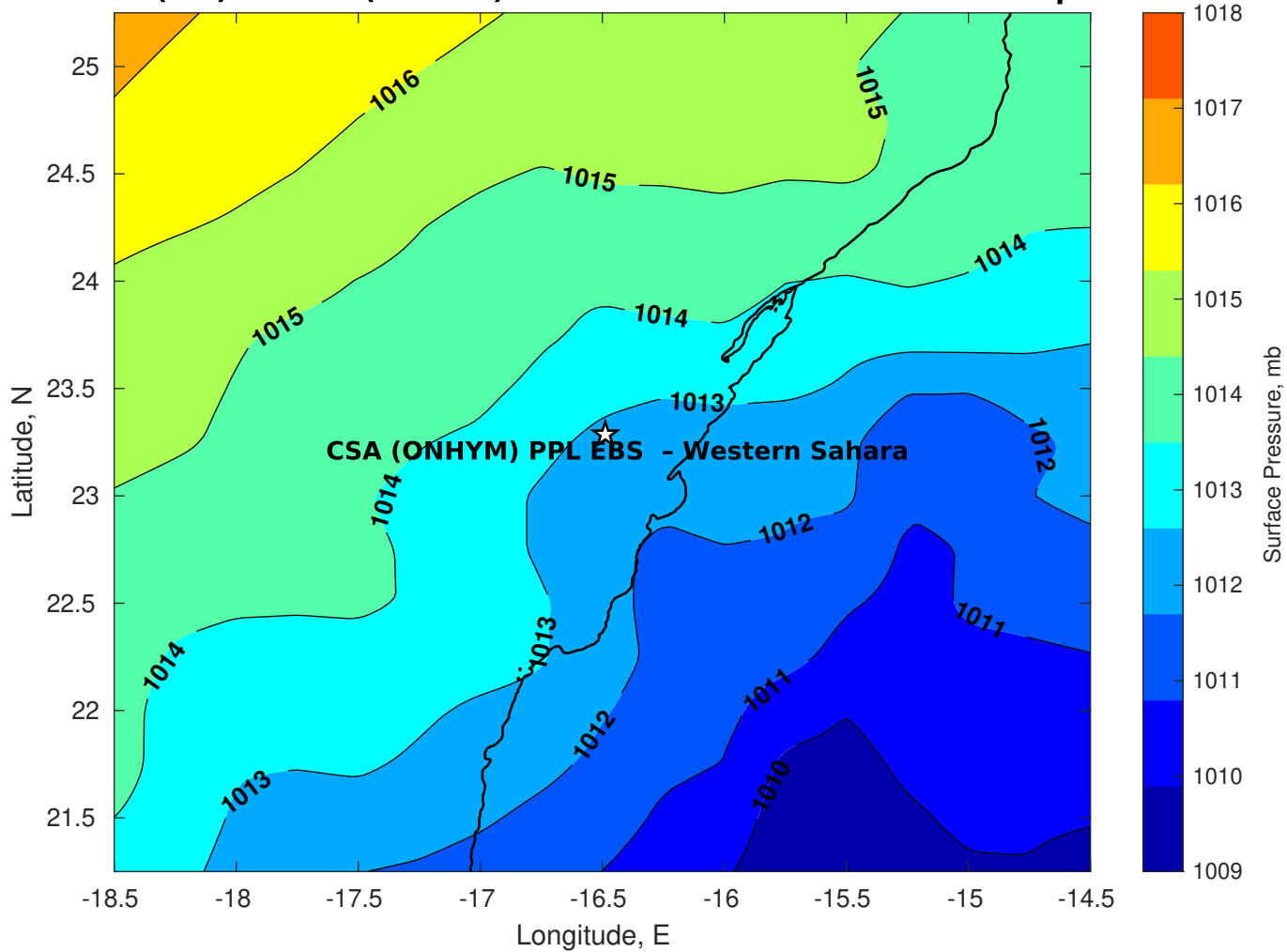
Surface Pressure (mb) for CSA (ONHYM) PPL EBS - Western Sahara at 30-Apr-2025 00:00:00
