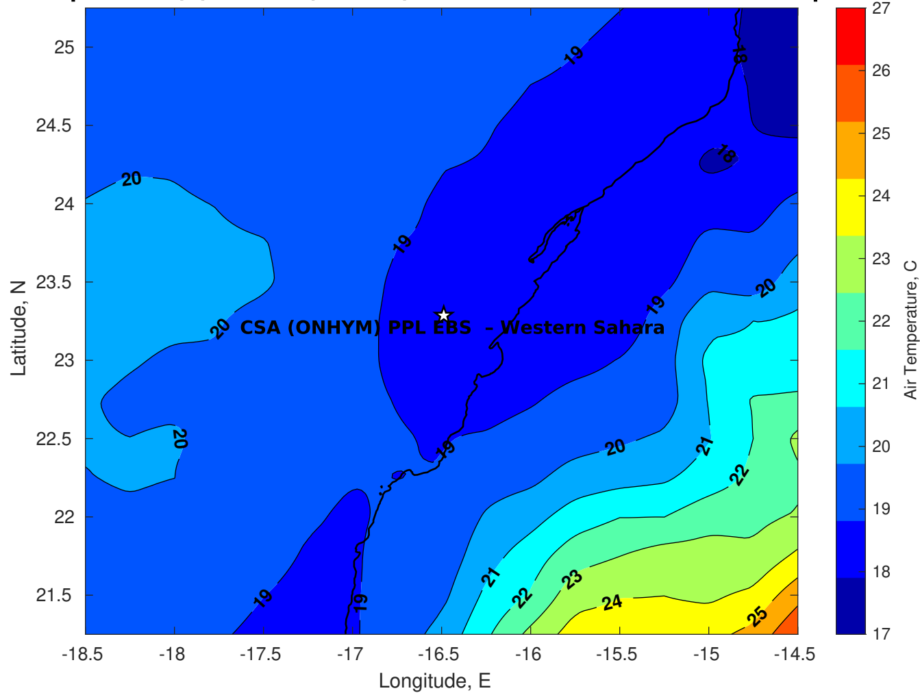
Air Temperature (C) for CSA (ONHYM) PPL EBS - Western Sahara at 29-Apr-2025
