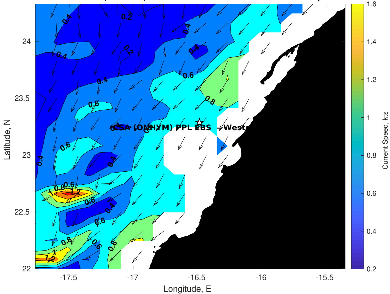
Surface Currents for CSA (ONHYM) PPL EBS - Western Sahara at 28-Apr-2025 00:00:00
