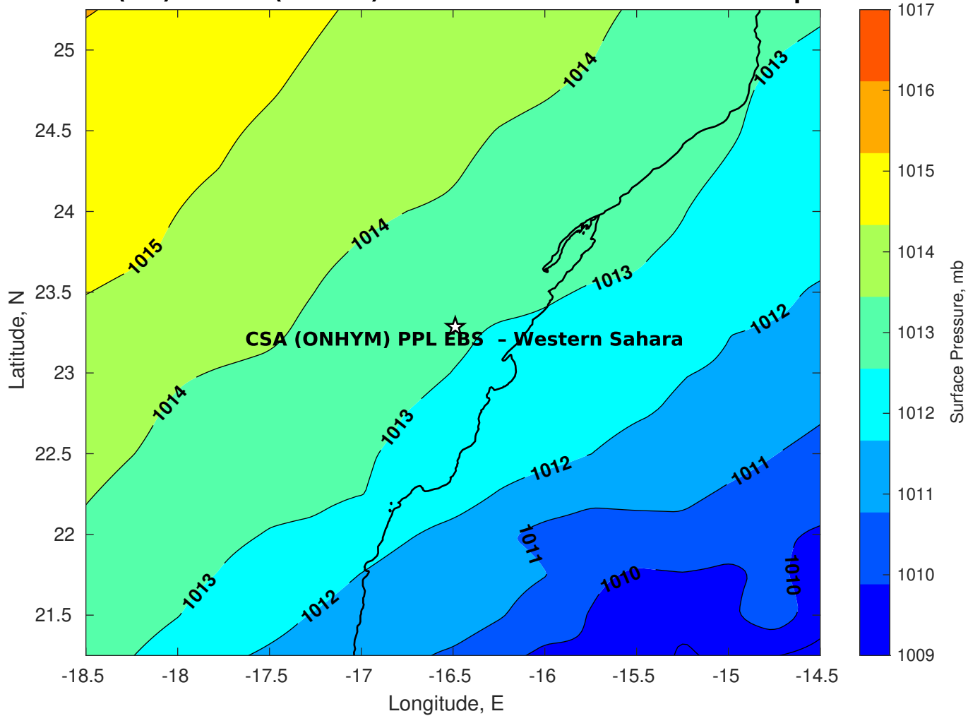
Surface Pressure (mb) for CSA (ONHYM) PPL EBS - Western Sahara at 29-Apr-2025 00:00:00
