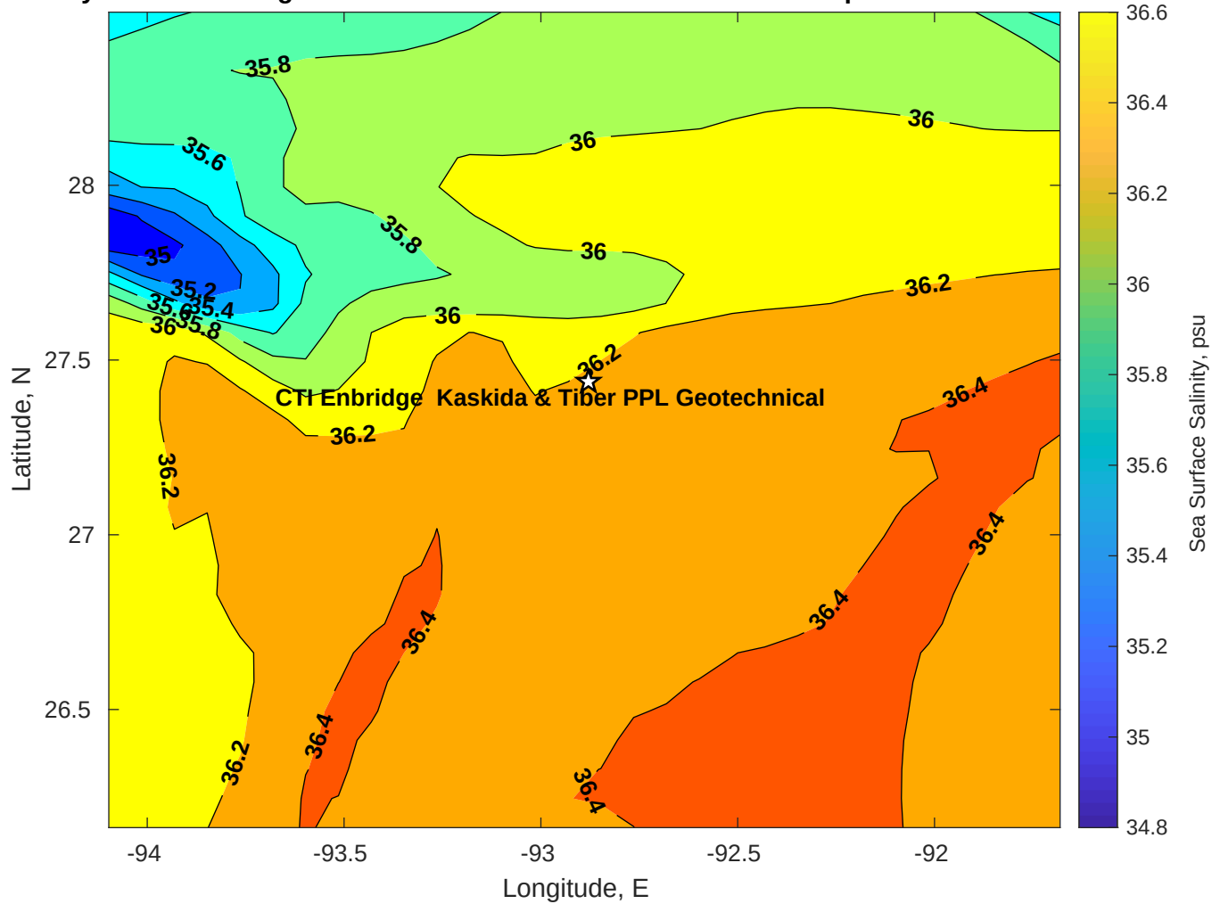
Surface Salinity for CTI Enbridge Kaskida & Tiber PPL Geotechnical at 28-Apr-2025 00:00:00
