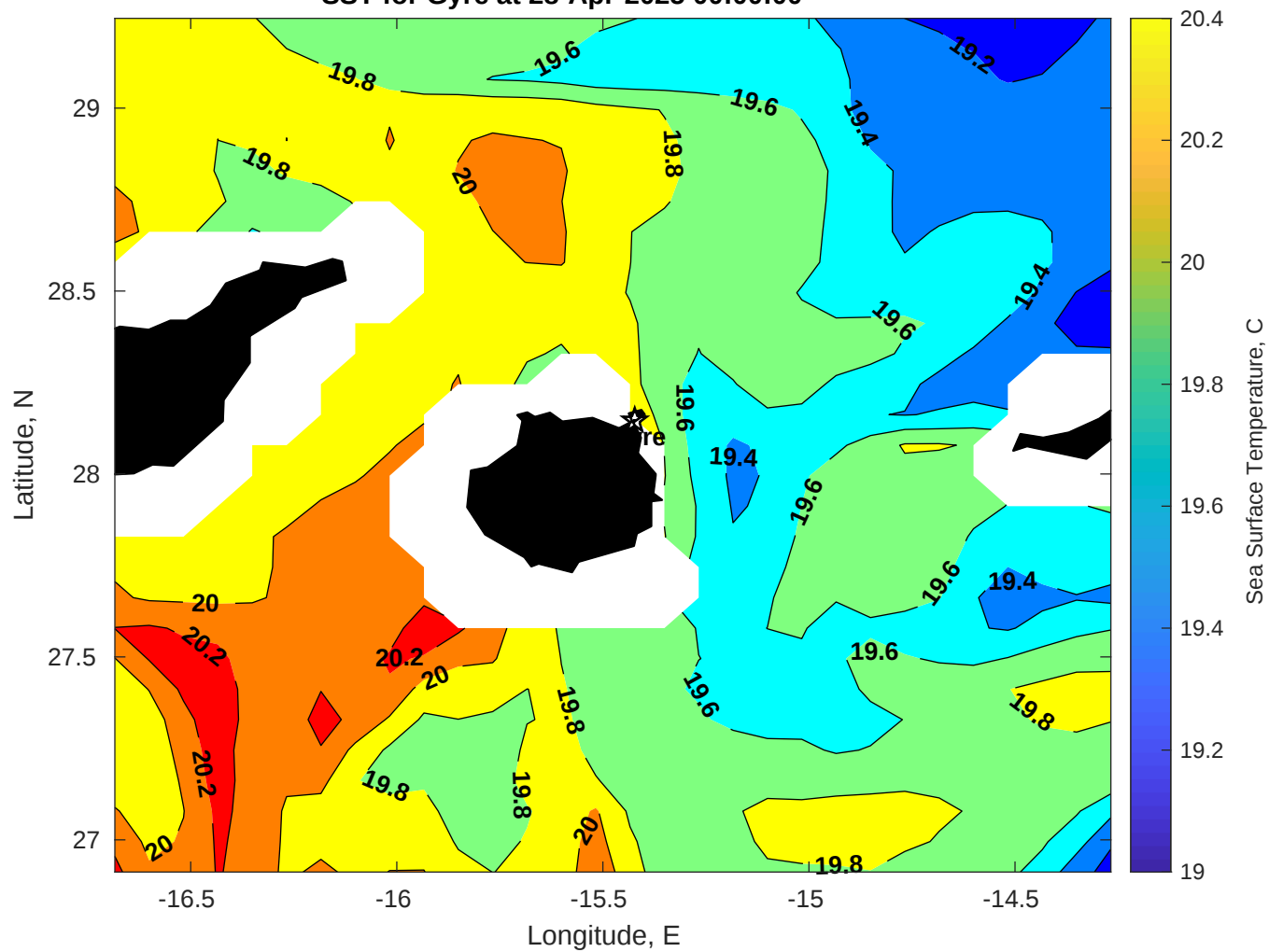
SST for Gyre at 28-Apr-2025 00:00:00
