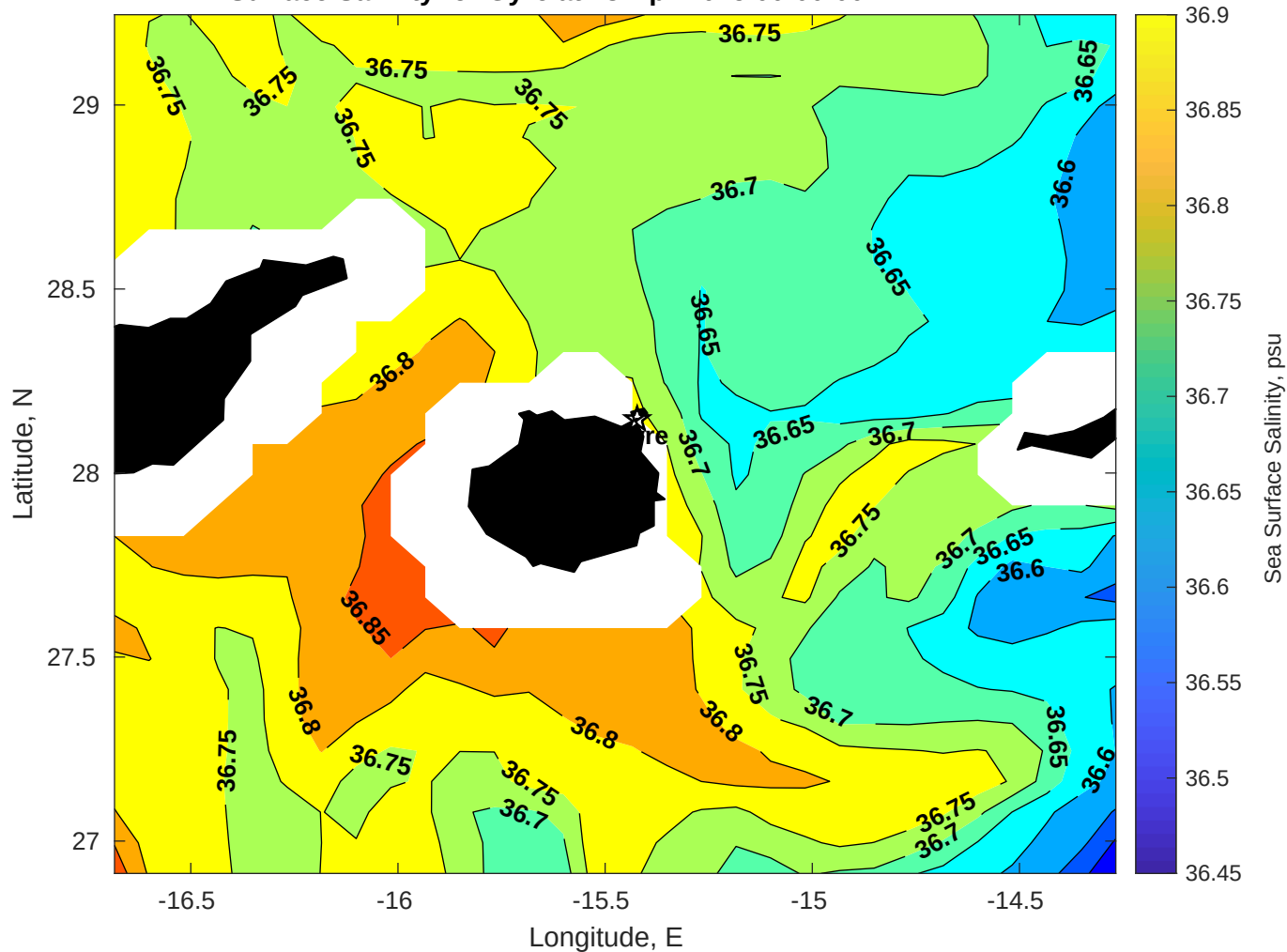
Surface Salinity for Gyre at 28-Apr-2025 00:00:00
