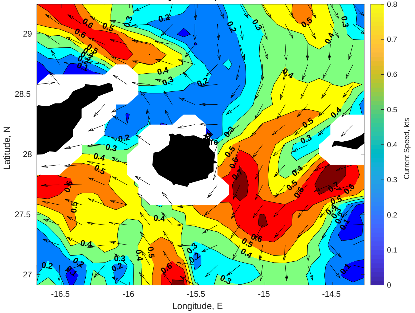
Surface Currents for Gyre at 28-Apr-2025 00:00:00
