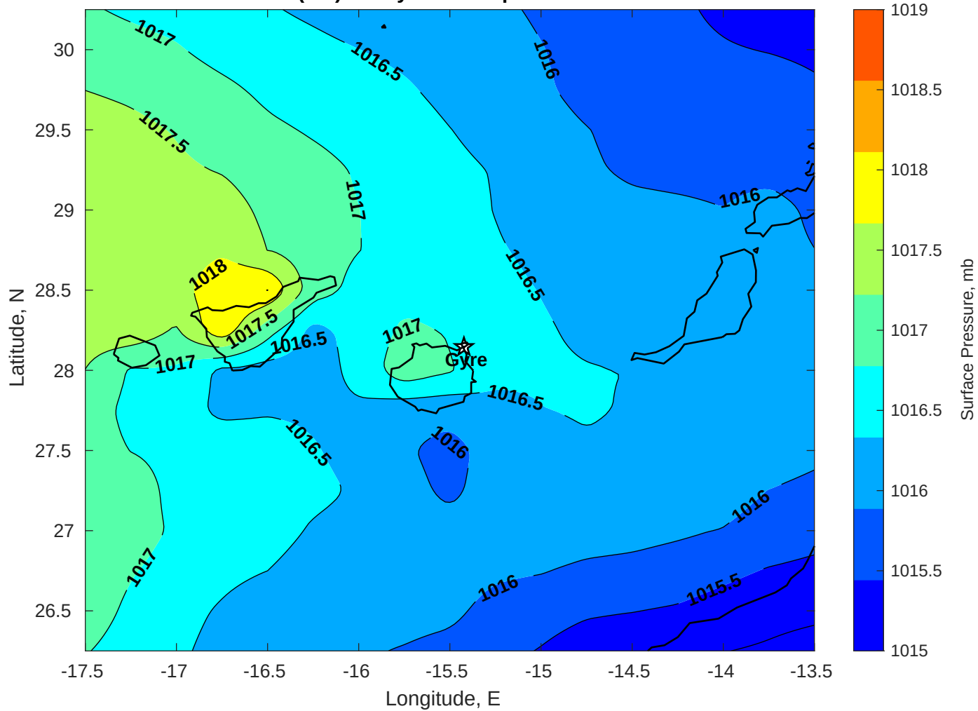
Surface Pressure (mb) for Gyre at 30-Apr-2025 00:00:00
