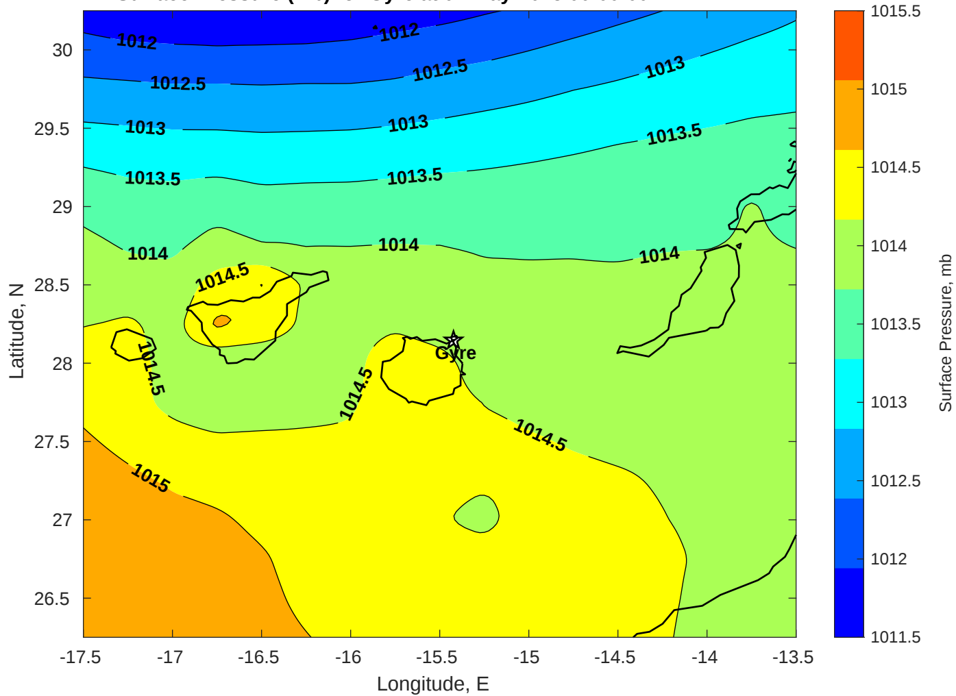
Surface Pressure (mb) for Gyre at 01-May-2025 00:00:00
