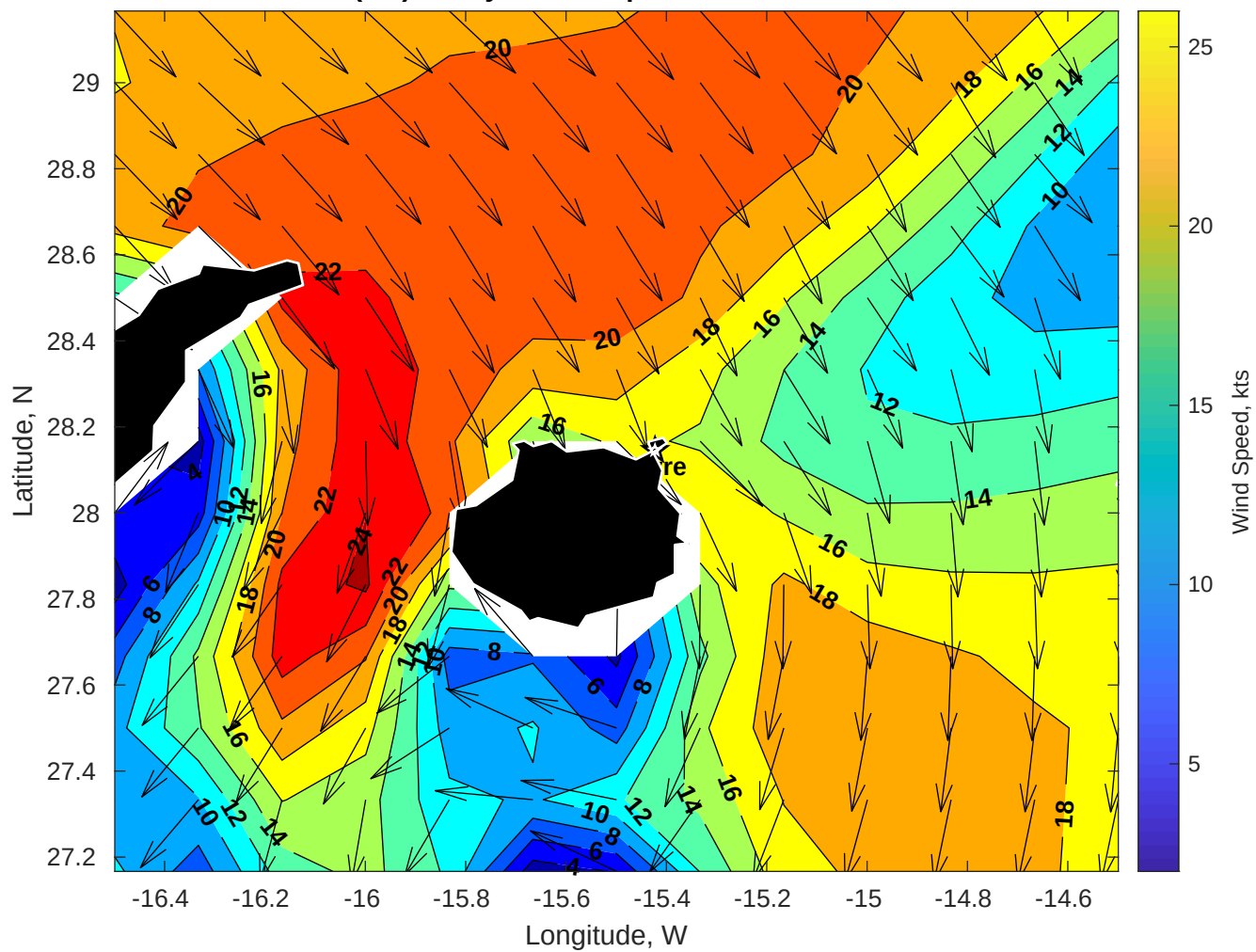
Winds (kts) for Gyre at 29-Apr-2025 09:00:00
