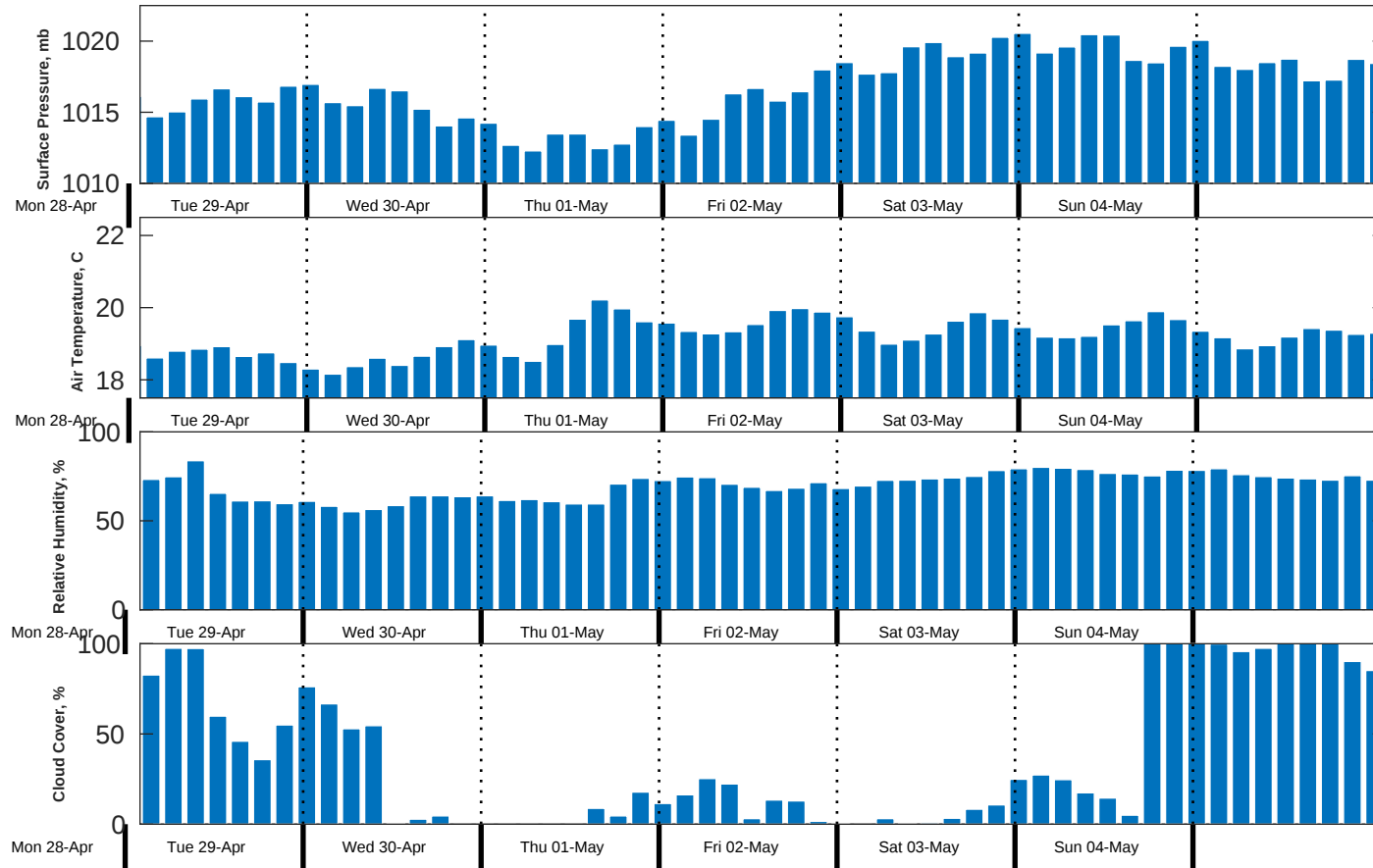
Met Forecast for Gyre from 28-Apr-2025 23:00:00 to 05-May-2025 23:00:00
