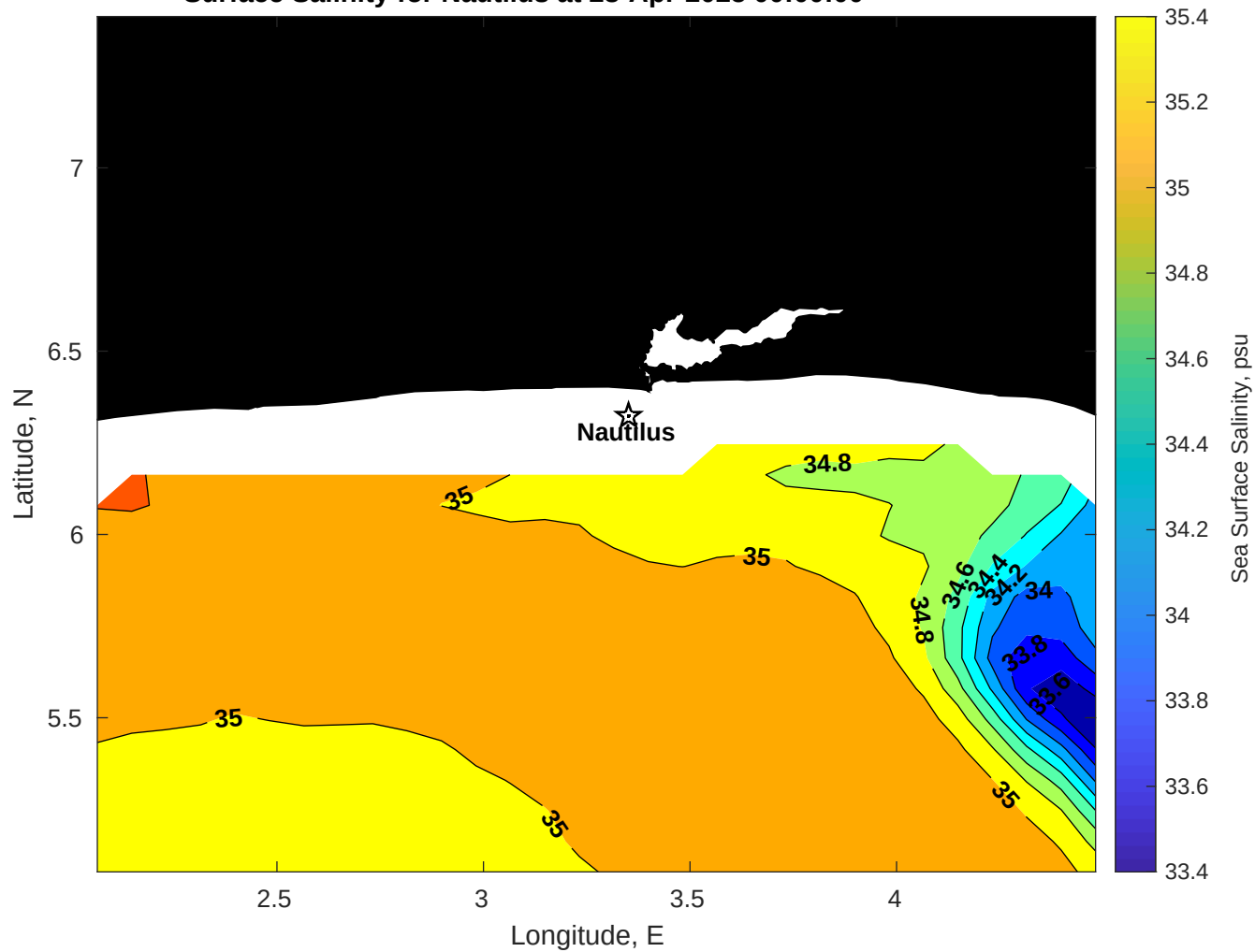
Surface Salinity for Nautilus at 28-Apr-2025 00:00:00
