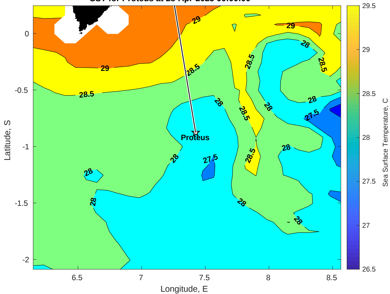
SST for Proteus at 28-Apr-2025 00:00:00
