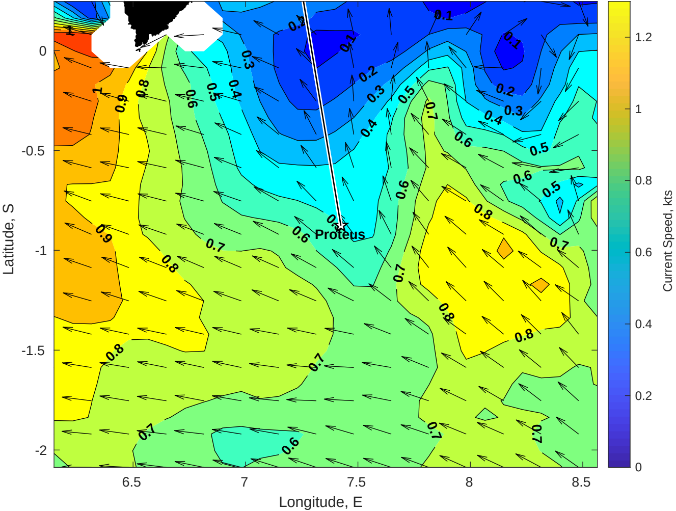
Surface Currents for Proteus at 28-Apr-2025 00:00:00
