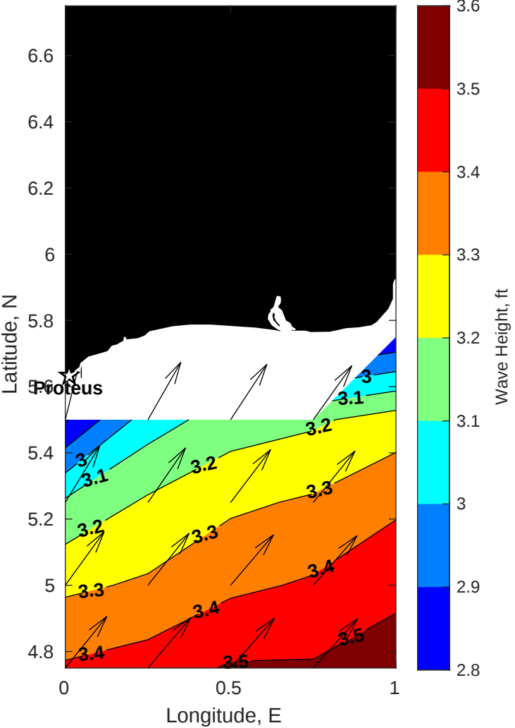
Wave Height (ft) for Proteus at 29-Apr-2025 09:00:00
