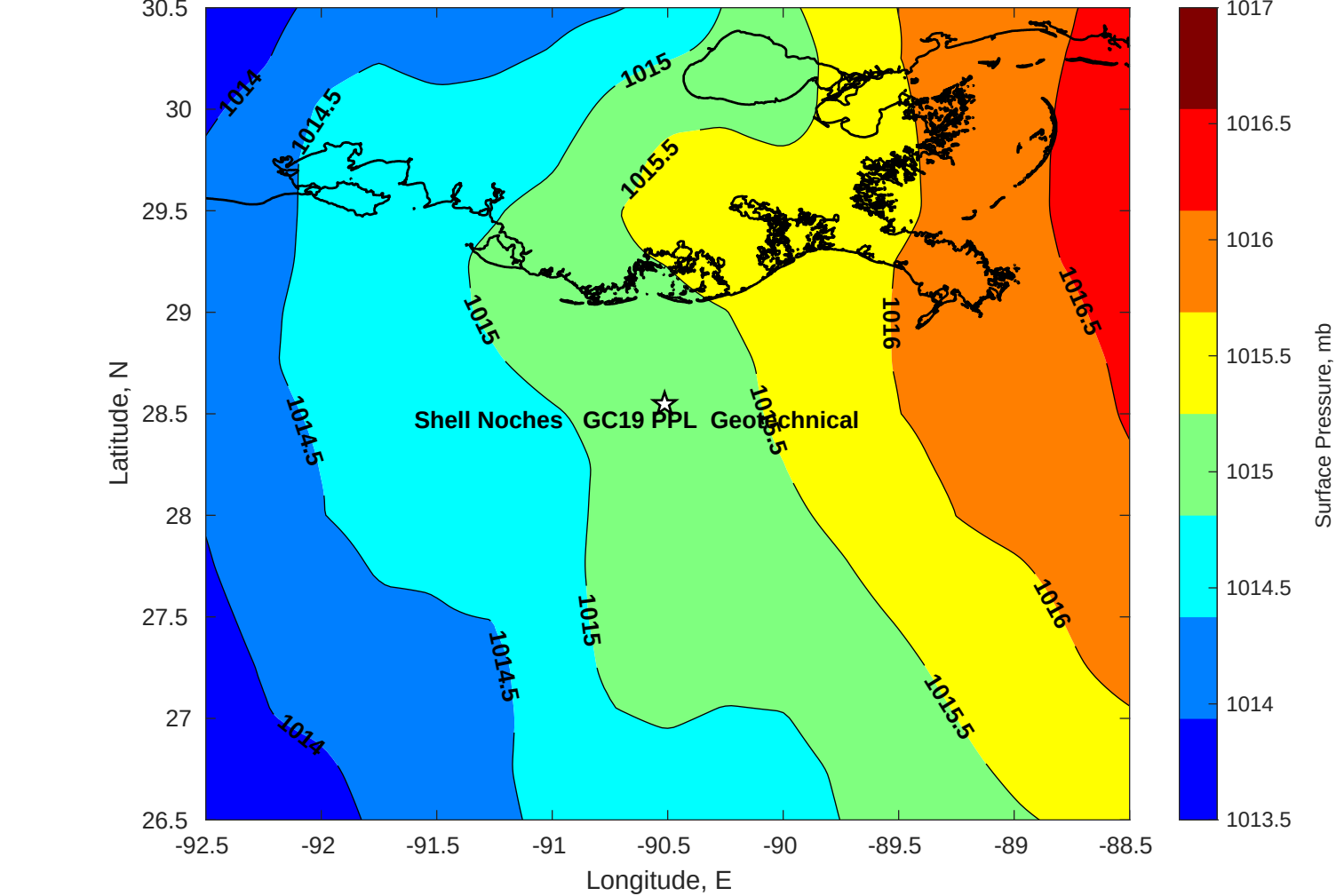
Surface Pressure (mb) for Shell Noches GC19 PPL Geotechnical at 01-May-2025 00:00:00
