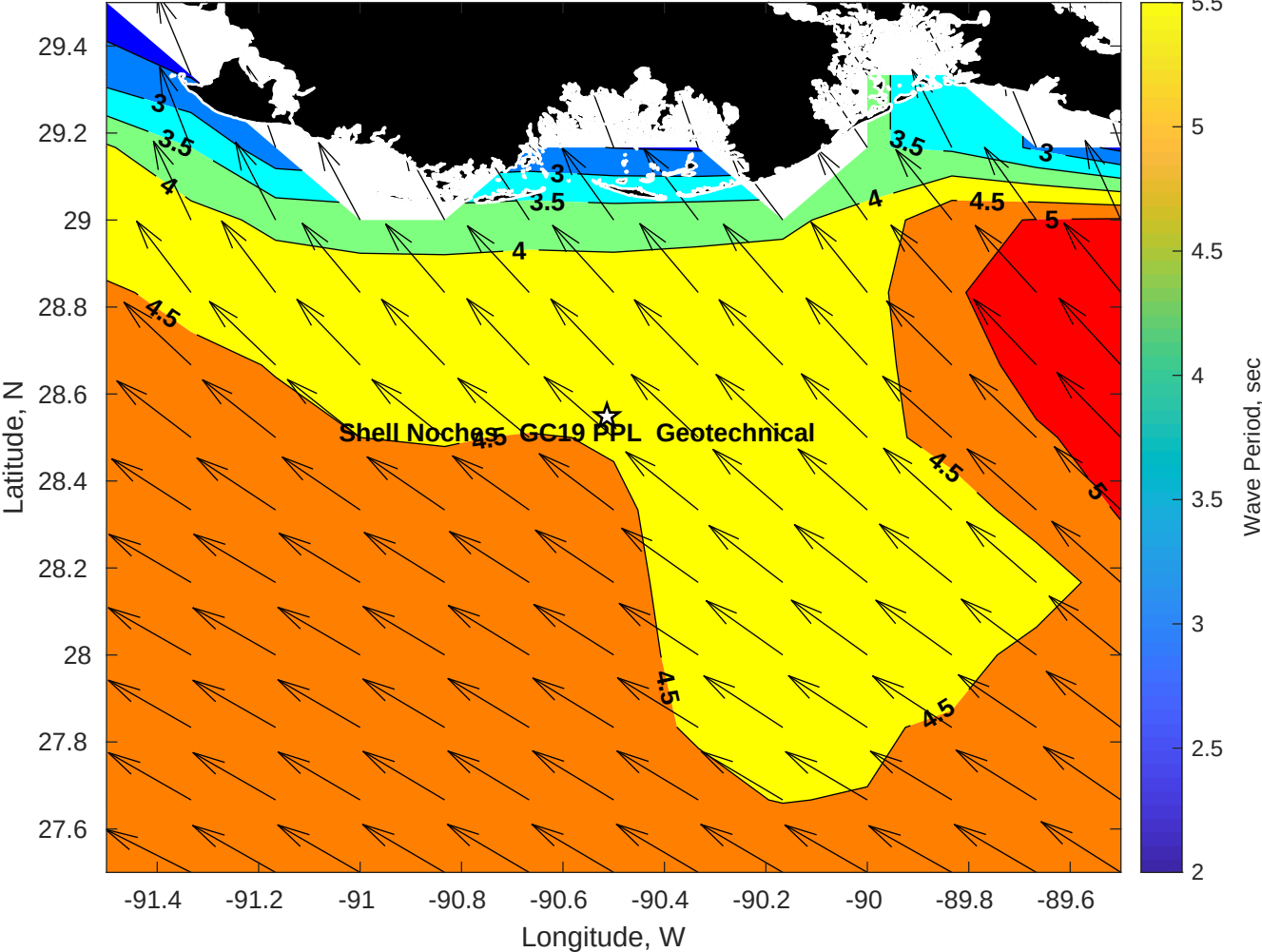
Wave Period (sec) for Shell Noches GC19 PPL Geotechnical at 29-Apr-2025 09:00:00
